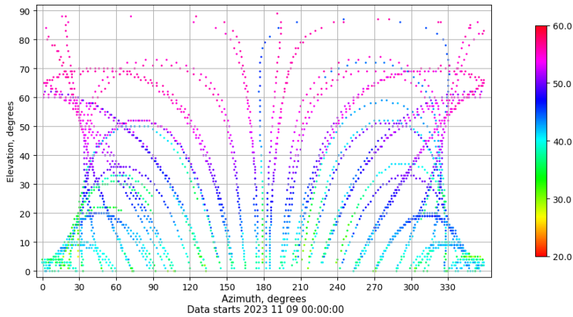
Azimuth-elevation plot for station XIXO. Signal to Noise S1C Data file XIXO00ESP_R_2023313.xtr
