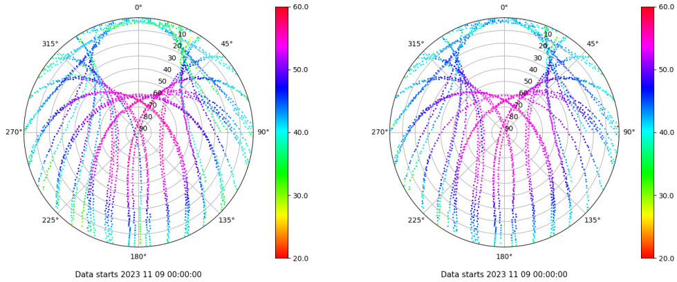
Skyplot for station XIXO. Signal to Noise S1C Data file XIXO00ESP_R_2023313.xtr Skyplot for station XIXO. Signal to Noise S2C Data file XIXO00ESP_R_2023313.xtr
