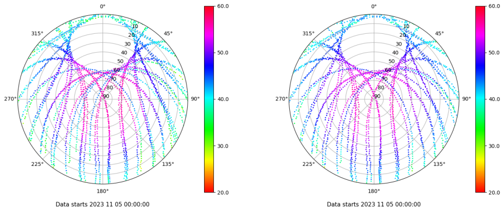
Skyplot for station XIXO. Signal to Noise S1C Data file XIXO00ESP_R_2023309.xtr Skyplot for station XIXO. Signal to Noise S2C Data file XIXO00ESP_R_2023309.xtr
