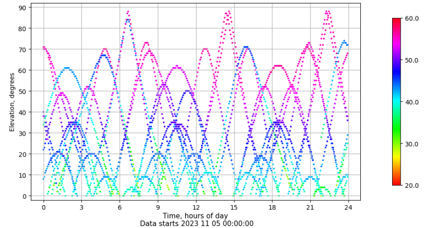
Time-elevation plot for station XIXO. Signal to Noise S1C Data file XIXO00ESP_R_2023309.xtr
