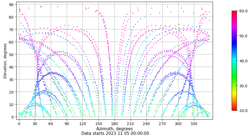
Azimuth-elevation plot for station XIXO. Signal to Noise S1C Data file XIXO00ESP_R_2023309.xtr
