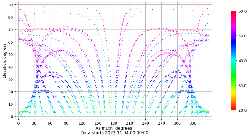
Azimuth-elevation plot for station XIXO. Signal to Noise S1C Data file XIXO00ESP_R_2023308.xtr
