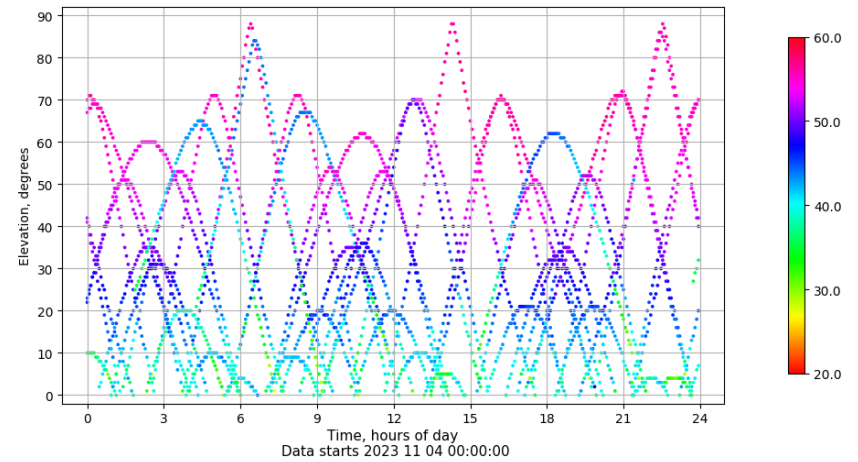
Time-elevation plot for station XIXO. Signal to Noise S1C Data file XIXO00ESP_R_2023308.xtr
