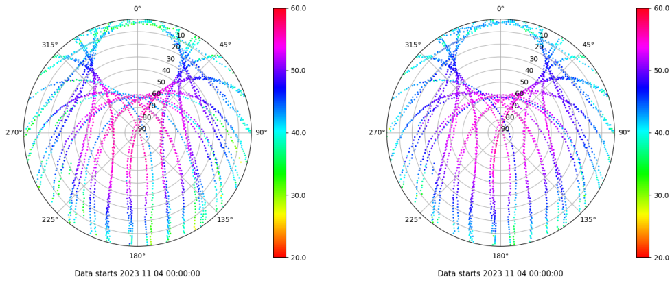
Skyplot for station XIXO. Signal to Noise S1C Data file XIXO00ESP_R_2023308.xtr Skyplot for station XIXO. Signal to Noise S2C Data file XIXO00ESP_R_2023308.xtr
