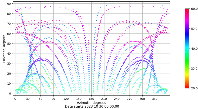
Azimuth-elevation plot for station XIXO. Signal to Noise S1C Data file XIXO00ESP_R_2023303.xtr
