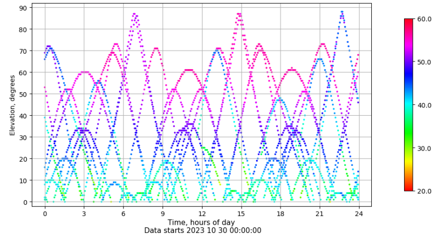
Time-elevation plot for station XIXO. Signal to Noise S1C Data file XIXO00ESP_R_2023303.xtr
