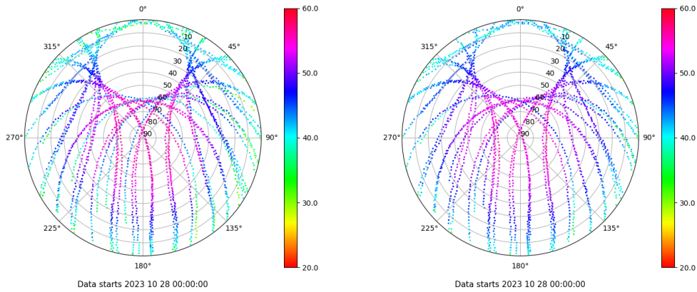
Skyplot for station XIXO. Signal to Noise S1C Data file XIXO00ESP_R_2023301.xtr Skyplot for station XIXO. Signal to Noise S2C Data file XIXO00ESP_R_2023301.xtr
