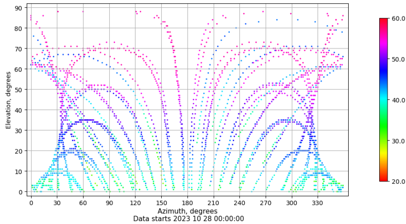
Azimuth-elevation plot for station XIXO. Signal to Noise S1C Data file XIXO00ESP_R_2023301.xtr
