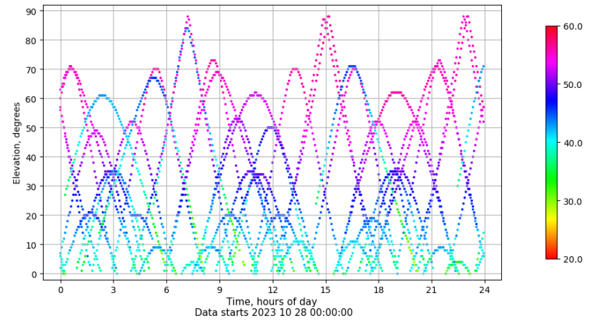
Time-elevation plot for station XIXO. Signal to Noise S1C Data file XIXO00ESP_R_2023301.xtr
