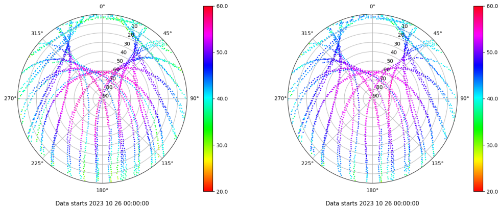
Skyplot for station XIXO. Signal to Noise S1C Data file XIXO00ESP_R_2023299.xtr Skyplot for station XIXO. Signal to Noise S2C Data file XIXO00ESP_R_2023299.xtr
