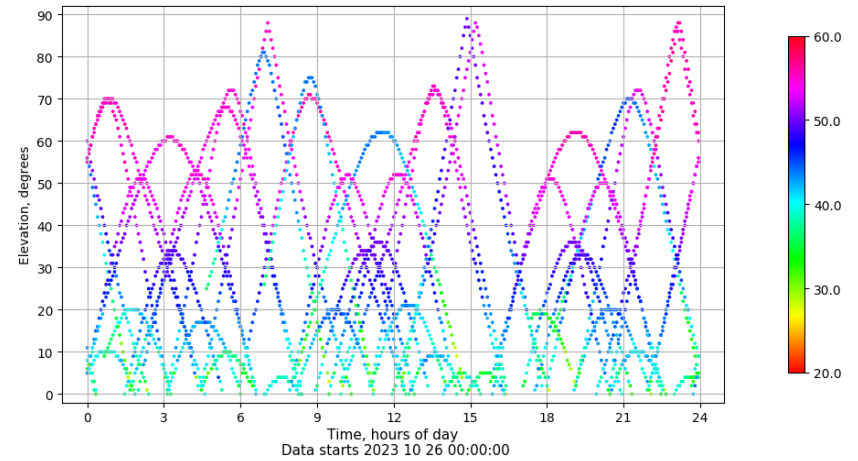
Time-elevation plot for station XIXO. Signal to Noise S1C Data file XIXO00ESP_R_2023299.xtr
