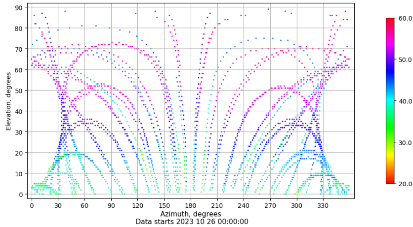
Azimuth-elevation plot for station XIXO. Signal to Noise S1C Data file XIXO00ESP_R_2023299.xtr
