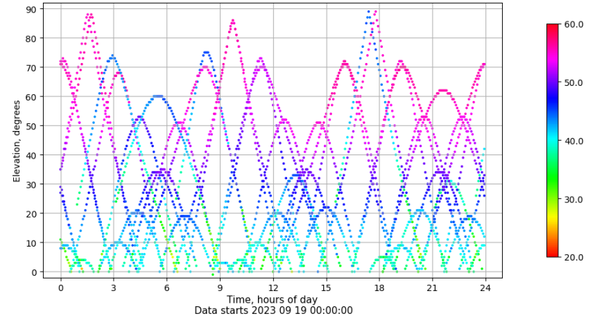
Time-elevation plot for station XIXO. Signal to Noise S1C Data file XIXO00ESP_R_2023262.xtr
