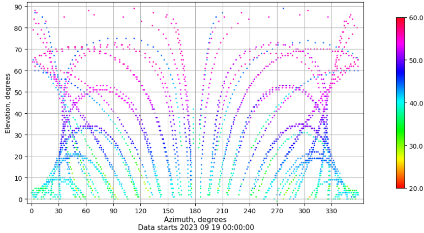
Azimuth-elevation plot for station XIXO. Signal to Noise S1C Data file XIXO00ESP_R_2023262.xtr
