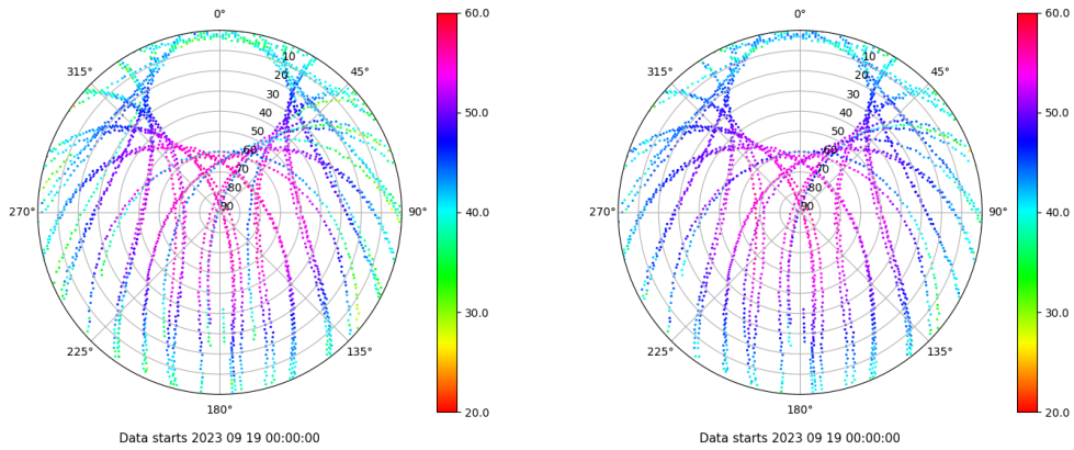
Skyplot for station XIXO. Signal to Noise S1C Data file XIXO00ESP_R_2023262.xtr Skyplot for station XIXO. Signal to Noise S2C Data file XIXO00ESP_R_2023262.xtr
