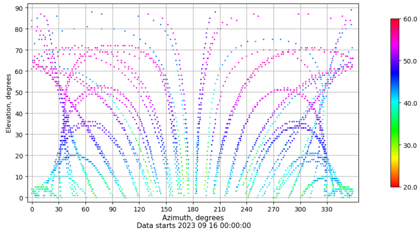
Azimuth-elevation plot for station XIXO. Signal to Noise S1C Data file XIXO00ESP_R_2023259.xtr
