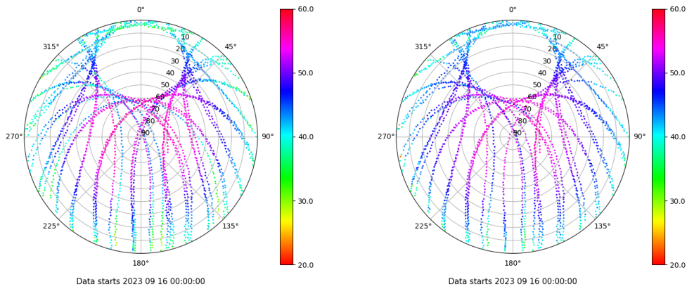
Skyplot for station XIXO. Signal to Noise S1C Data file XIXO00ESP_R_2023259.xtr Skyplot for station XIXO. Signal to Noise S2C Data file XIXO00ESP_R_2023259.xtr
