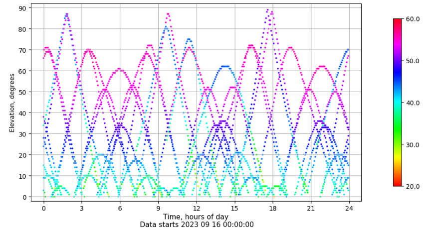
Time-elevation plot for station XIXO. Signal to Noise S1C Data file XIXO00ESP_R_2023259.xtr
