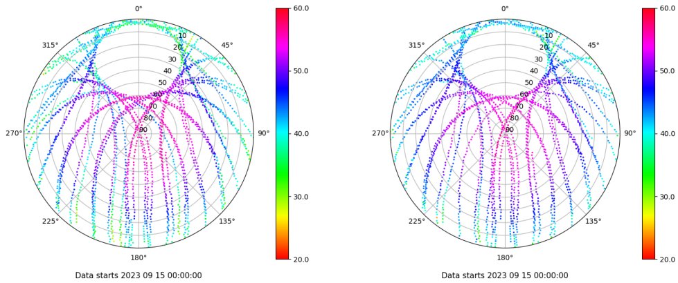
Skyplot for station XIXO. Signal to Noise S1C Data file XIXO00ESP_R_2023258.xtr Skyplot for station XIXO. Signal to Noise S2C Data file XIXO00ESP_R_2023258.xtr
