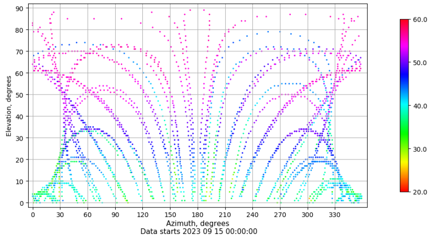
Azimuth-elevation plot for station XIXO. Signal to Noise S1C Data file XIXO00ESP_R_2023258.xtr
