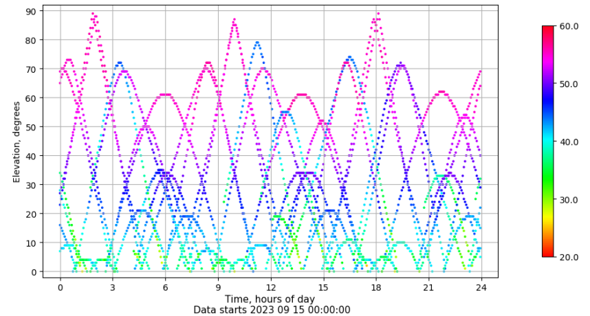
Time-elevation plot for station XIXO. Signal to Noise S1C Data file XIXO00ESP_R_2023258.xtr
