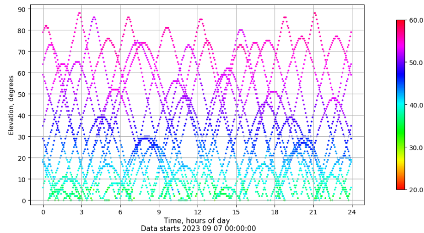
Time-elevation plot for station XIXO. Signal to Noise S1C Data file XIXO00ESP_R_2023250.xtr
