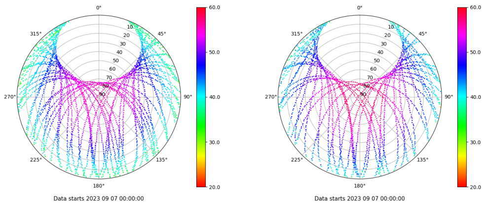
Skyplot for station XIXO. Signal to Noise S1C Data file XIXO00ESP_R_2023250.xtr Skyplot for station XIXO. Signal to Noise S2S Data file XIXO00ESP_R_2023250.xtr
