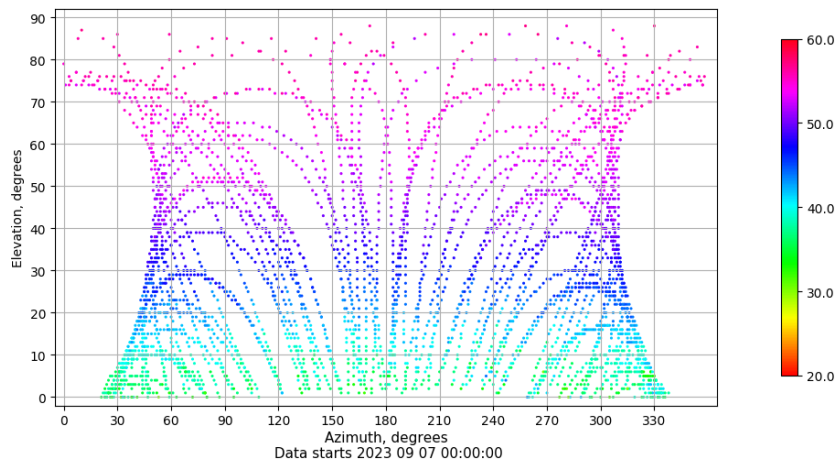
Azimuth-elevation plot for station XIXO. Signal to Noise S1C Data file XIXO00ESP_R_2023250.xtr
