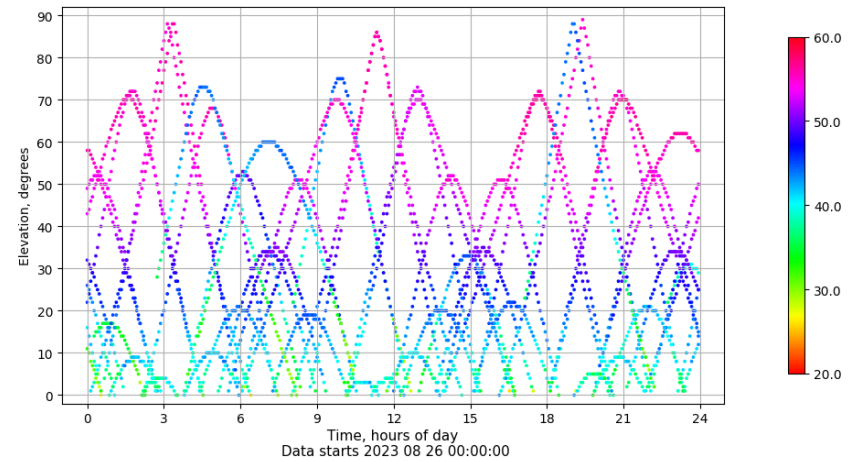
Time-elevation plot for station XIXO. Signal to Noise S1C Data file XIXO00ESP_R_2023238.xtr
