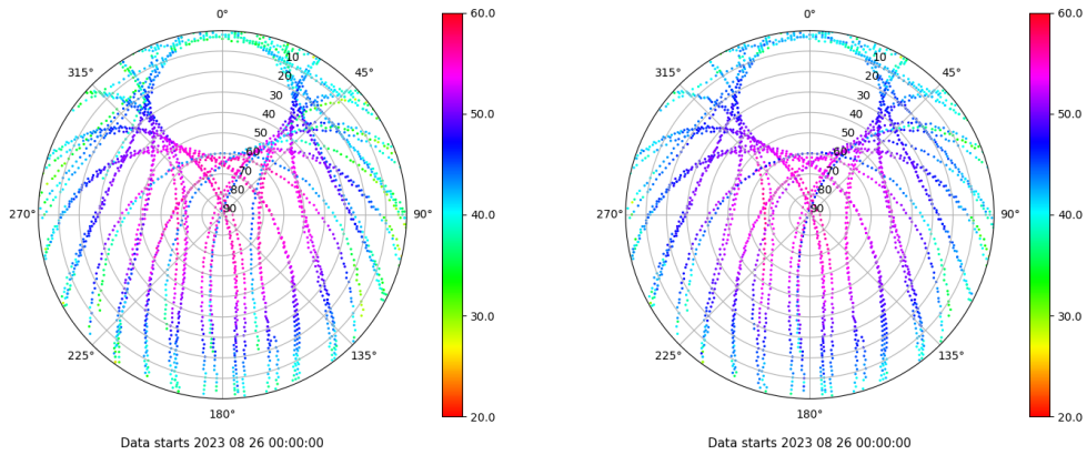
Skyplot for station XIXO. Signal to Noise S1C Data file XIXO00ESP_R_2023238.xtr Skyplot for station XIXO. Signal to Noise S2C Data file XIXO00ESP_R_2023238.xtr
