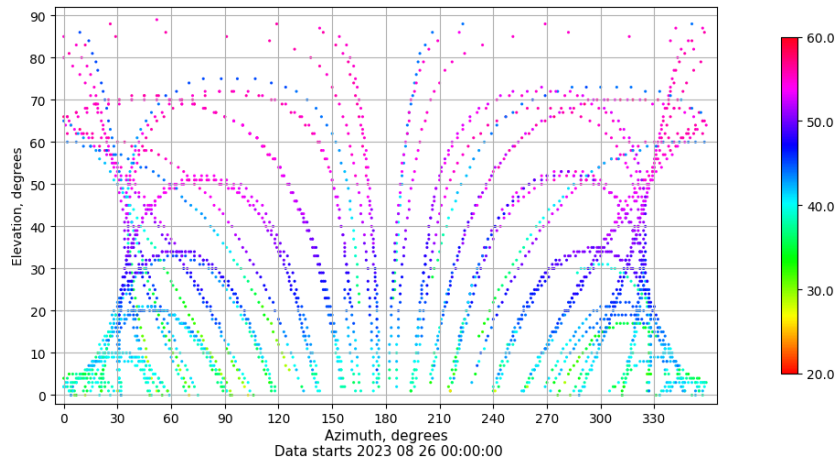
Azimuth-elevation plot for station XIXO. Signal to Noise S1C Data file XIXO00ESP_R_2023238.xtr
