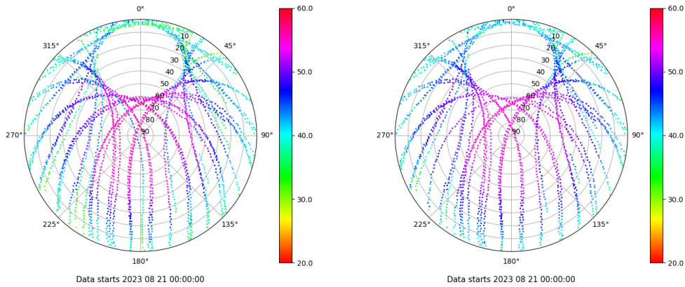
Skyplot for station XIXO. Signal to Noise S1C Data file XIXO00ESP_R_2023233.xtr Skyplot for station XIXO. Signal to Noise S2C Data file XIXO00ESP_R_2023233.xtr
