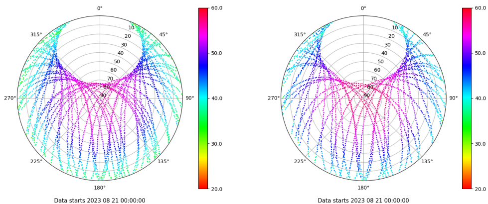
Skyplot for station XIXO. Signal to Noise S1C Data file XIXO00ESP_R_2023233.xtr Skyplot for station XIXO. Signal to Noise S2S Data file XIXO00ESP_R_2023233.xtr
