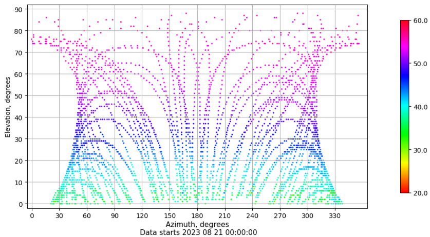
Azimuth-elevation plot for station XIXO. Signal to Noise S1C Data file XIXO00ESP_R_2023233.xtr
