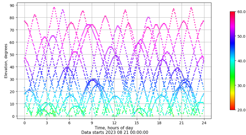
Time-elevation plot for station XIXO. Signal to Noise S1C Data file XIXO00ESP_R_2023233.xtr
