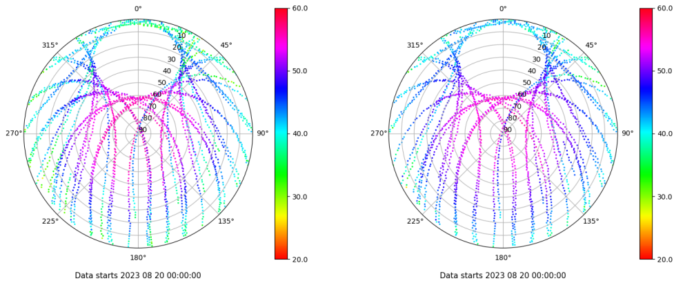
Skyplot for station XIXO. Signal to Noise S1C Data file XIXO00ESP_R_2023232.xtr Skyplot for station XIXO. Signal to Noise S2C Data file XIXO00ESP_R_2023232.xtr
