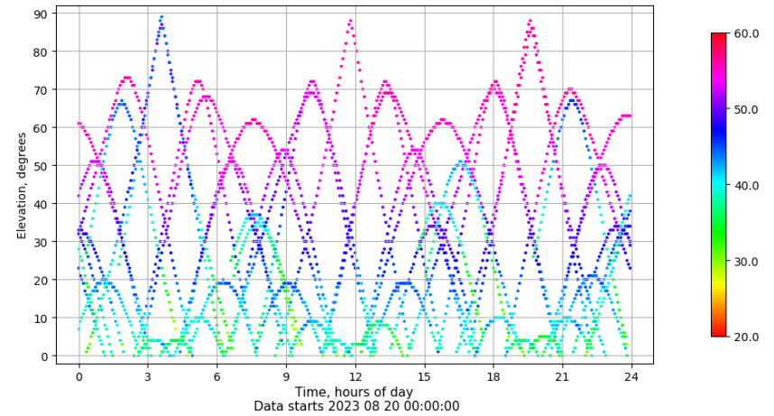
Time-elevation plot for station XIXO. Signal to Noise S1C Data file XIXO00ESP_R_2023232.xtr
