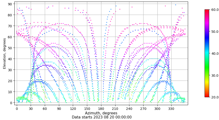
Azimuth-elevation plot for station XIXO. Signal to Noise S1C Data file XIXO00ESP_R_2023232.xtr
