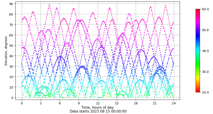
Time-elevation plot for station XIXO. Signal to Noise S1C Data file XIXO00ESP_R_2023227.xtr
