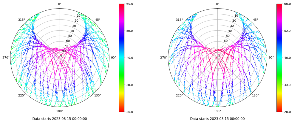
Skyplot for station XIXO. Signal to Noise S1C Data file XIXO00ESP_R_2023227.xtr Skyplot for station XIXO. Signal to Noise S2S Data file XIXO00ESP_R_2023227.xtr
