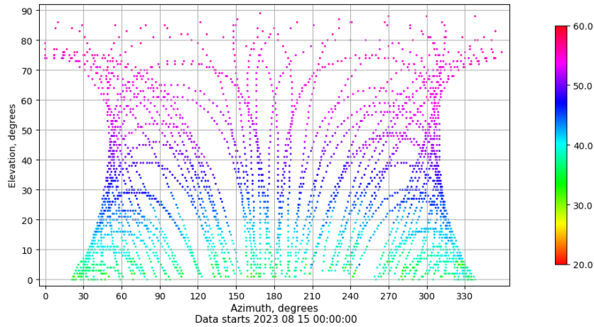
Azimuth-elevation plot for station XIXO. Signal to Noise S1C Data file XIXO00ESP_R_2023227.xtr
