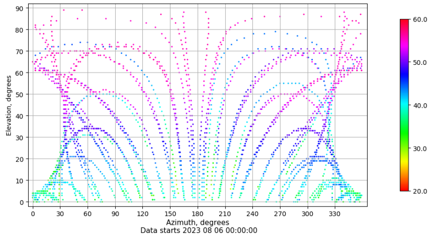
Azimuth-elevation plot for station XIXO. Signal to Noise S1C Data file XIXO00ESP_R_2023218.xtr
