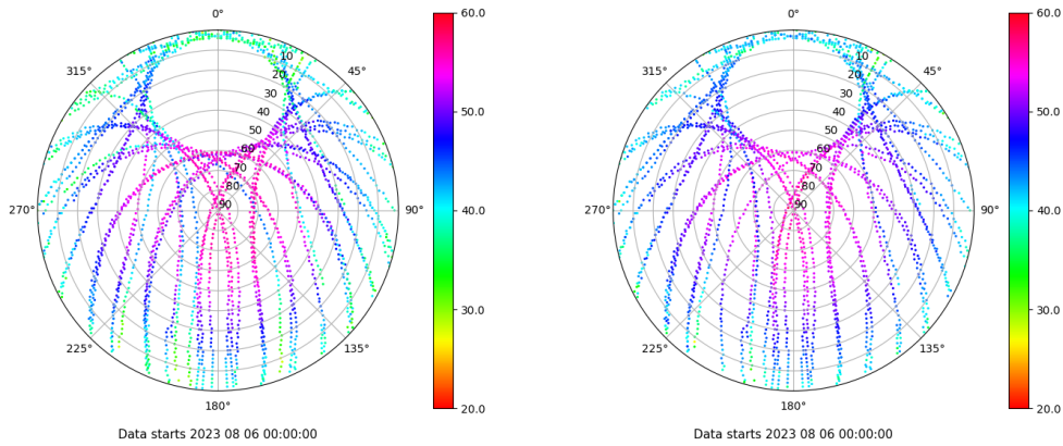
Skyplot for station XIXO. Signal to Noise S1C Data file XIXO00ESP_R_2023218.xtr Skyplot for station XIXO. Signal to Noise S2C Data file XIXO00ESP_R_2023218.xtr
