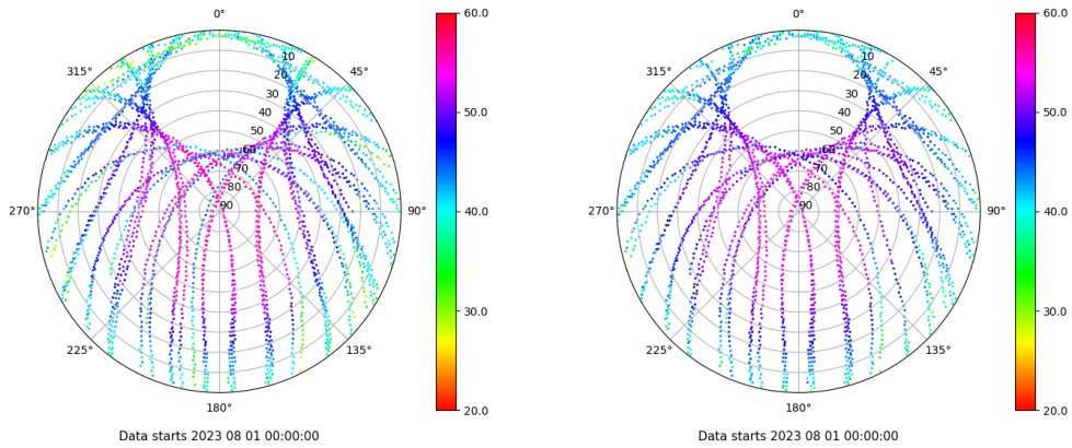
Skyplot for station XIXO. Signal to Noise S1C Data file XIXO00ESP_R_2023213.xtr Skyplot for station XIXO. Signal to Noise S2C Data file XIXO00ESP_R_2023213.xtr
