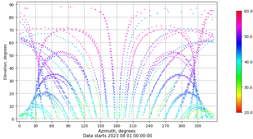
Azimuth-elevation plot for station XIXO. Signal to Noise S1C Data file XIXO00ESP_R_2023213.xtr
