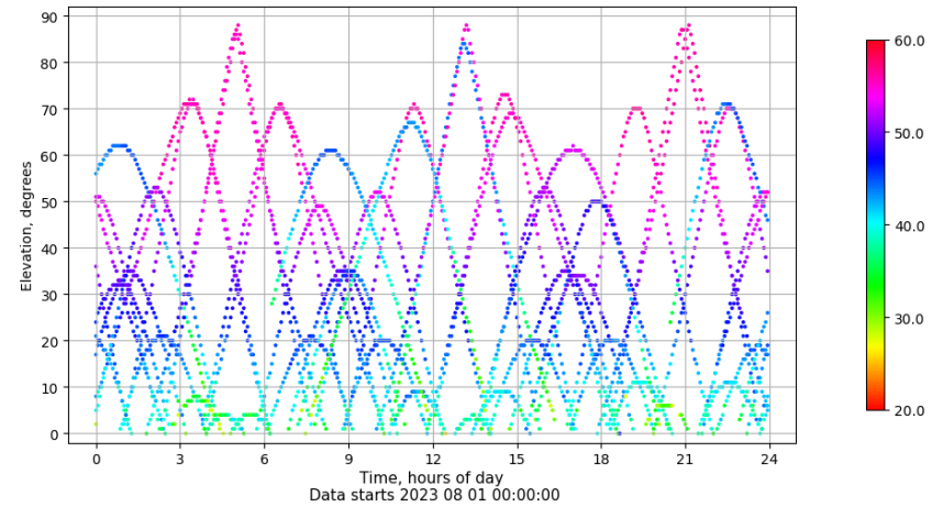
Time-elevation plot for station XIXO. Signal to Noise S1C Data file XIXO00ESP_R_2023213.xtr
