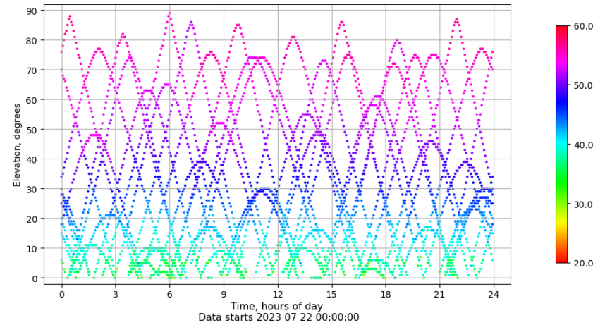
Time-elevation plot for station XIXO. Signal to Noise S1C Data file XIXO00ESP_R_2023203.xtr
