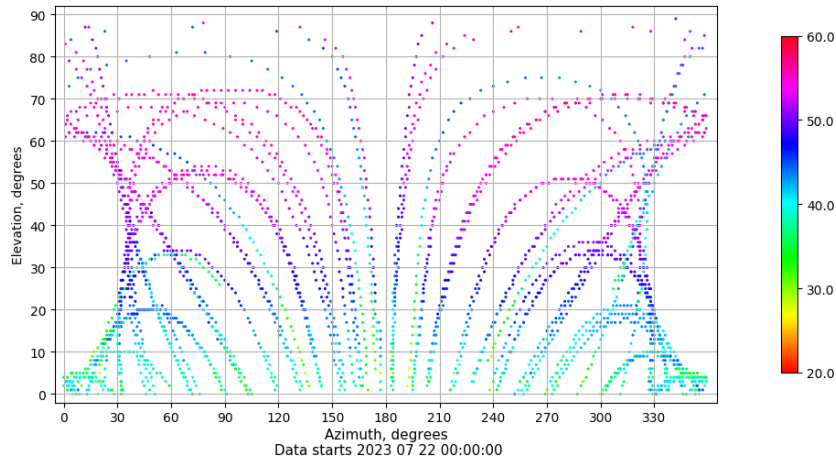
Azimuth-elevation plot for station XIXO. Signal to Noise S1C Data file XIXO00ESP_R_2023203.xtr
