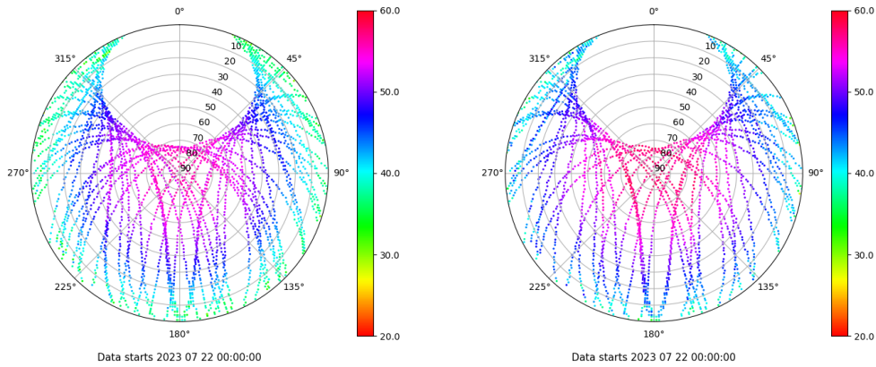
Skyplot for station XIXO. Signal to Noise S1C Data file XIXO00ESP_R_2023203.xtr Skyplot for station XIXO. Signal to Noise S2S Data file XIXO00ESP_R_2023203.xtr
