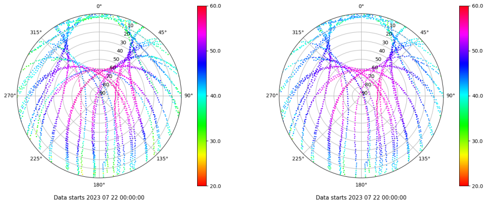
Skyplot for station XIXO. Signal to Noise S1C Data file XIXO00ESP_R_2023203.xtr Skyplot for station XIXO. Signal to Noise S2C Data file XIXO00ESP_R_2023203.xtr
