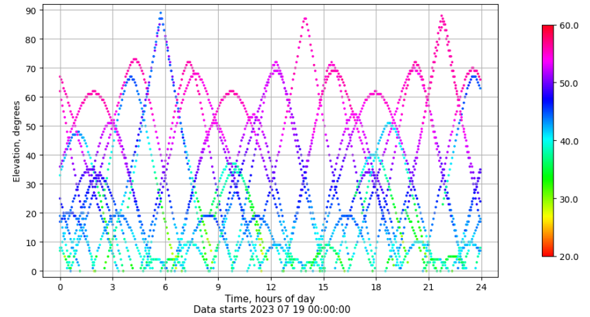
Time-elevation plot for station XIXO. Signal to Noise S1C Data file XIXO00ESP_R_2023200.xtr
