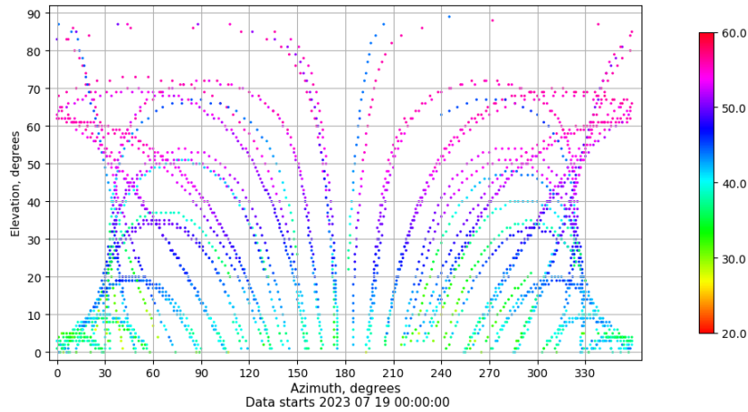
Azimuth-elevation plot for station XIXO. Signal to Noise S1C Data file XIXO00ESP_R_2023200.xtr
