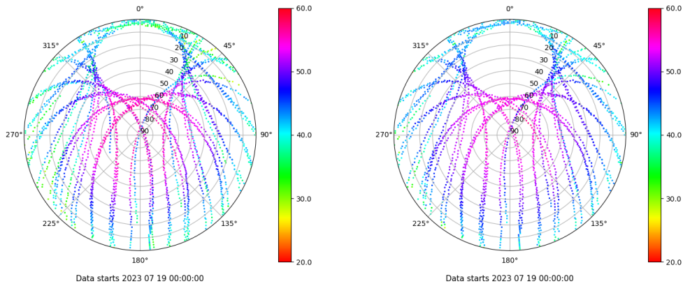
Skyplot for station XIXO. Signal to Noise S1C Data file XIXO00ESP_R_2023200.xtr Skyplot for station XIXO. Signal to Noise S2C Data file XIXO00ESP_R_2023200.xtr
