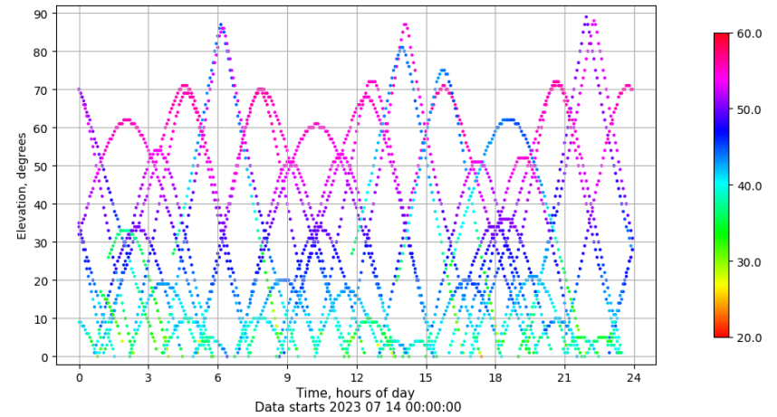
Time-elevation plot for station XIXO. Signal to Noise S1C Data file XIXO00ESP_R_2023195.xtr
