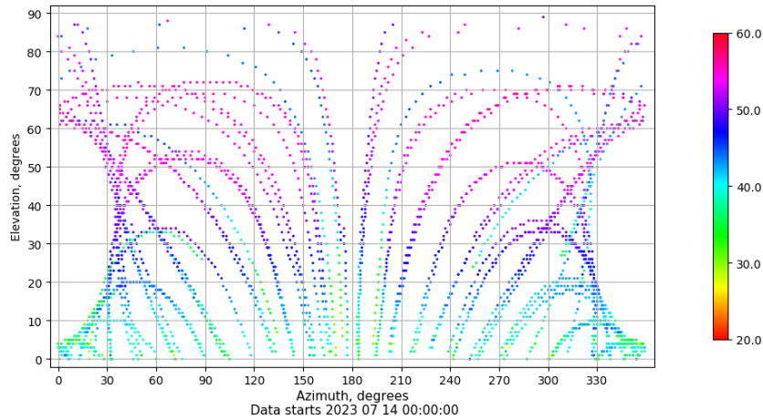
Azimuth-elevation plot for station XIXO. Signal to Noise S1C Data file XIXO00ESP_R_2023195.xtr
