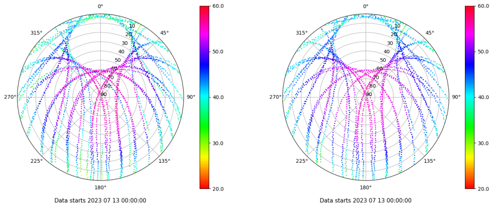
Skyplot for station XIXO. Signal to Noise S1C Data file XIXO00ESP_R_2023194.xtr Skyplot for station XIXO. Signal to Noise S2C Data file XIXO00ESP_R_2023194.xtr
