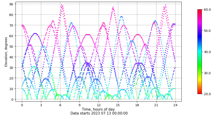
Time-elevation plot for station XIXO. Signal to Noise S1C Data file XIXO00ESP_R_2023194.xtr
