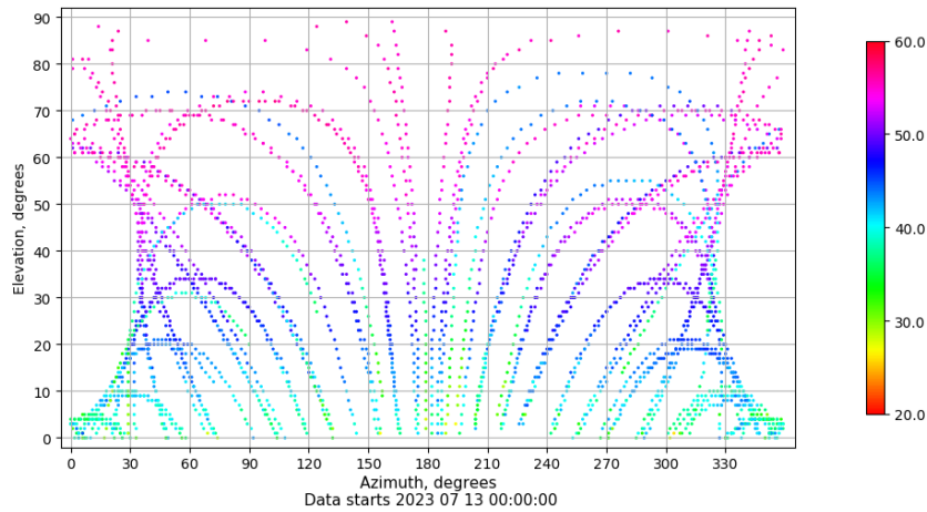
Azimuth-elevation plot for station XIXO. Signal to Noise S1C Data file XIXO00ESP_R_2023194.xtr
