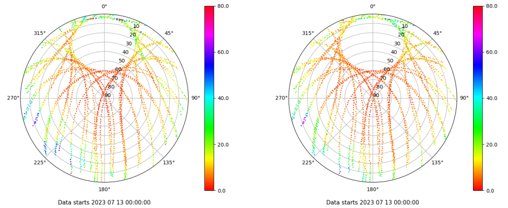
Skyplot for station XIXO. Parameter M1C Data file XIXO00ESP_R_2023194.xtr Skyplot for station XIXO. Parameter M2C Data file XIXO00ESP_R_2023194.xtr
