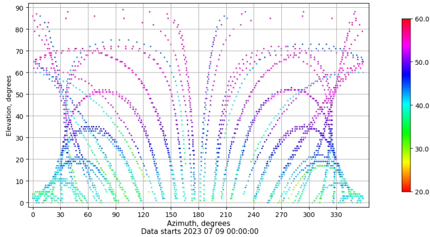
Azimuth-elevation plot for station XIXO. Signal to Noise S1C Data file XIXO00ESP_R_2023190.xtr
