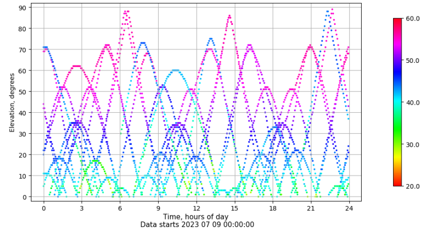
Time-elevation plot for station XIXO. Signal to Noise S1C Data file XIXO00ESP_R_2023190.xtr
