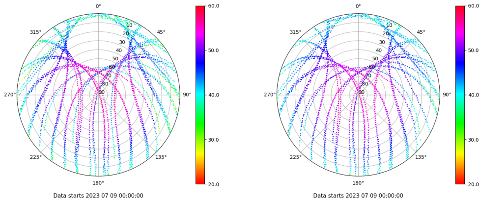
Skyplot for station XIXO. Signal to Noise S1C Data file XIXO00ESP_R_2023190.xtr Skyplot for station XIXO. Signal to Noise S2C Data file XIXO00ESP_R_2023190.xtr
