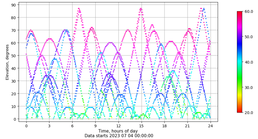
Time-elevation plot for station XIXO. Signal to Noise S1C Data file XIXO00ESP_R_2023185.xtr
