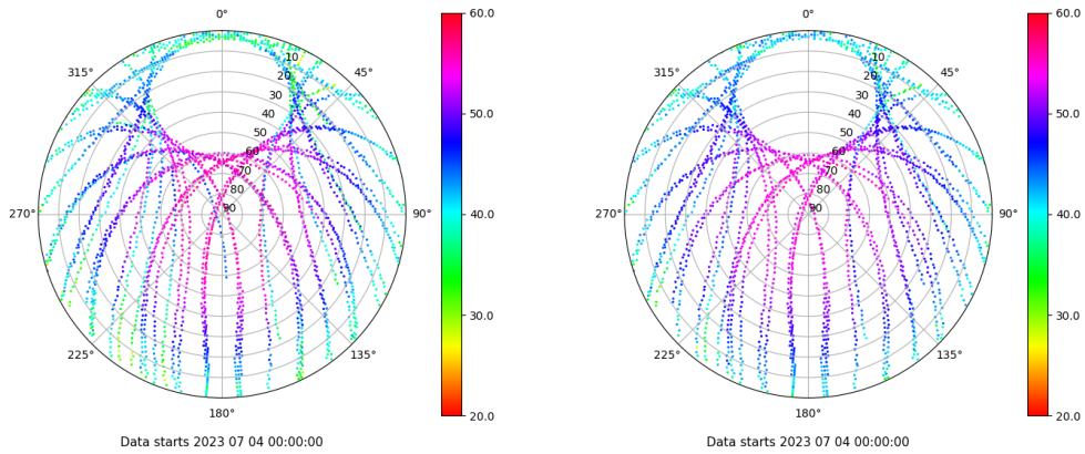
Skyplot for station XIXO. Signal to Noise S1C Data file XIXO00ESP_R_2023185.xtr Skyplot for station XIXO. Signal to Noise S2C Data file XIXO00ESP_R_2023185.xtr
