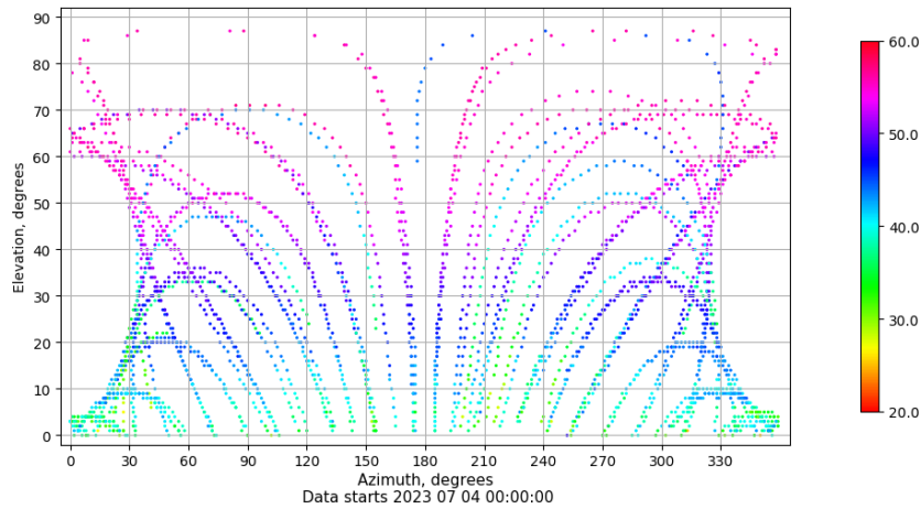
Azimuth-elevation plot for station XIXO. Signal to Noise S1C Data file XIXO00ESP_R_2023185.xtr
