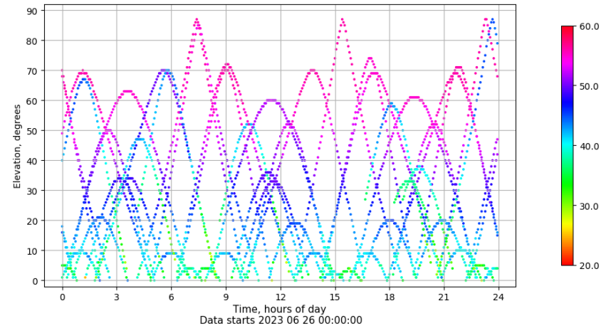
Time-elevation plot for station XIXO. Signal to Noise S1C Data file XIXO00ESP_R_2023177.xtr
