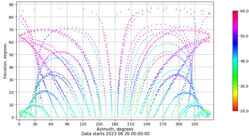
Azimuth-elevation plot for station XIXO. Signal to Noise S1C Data file XIXO00ESP_R_2023177.xtr
