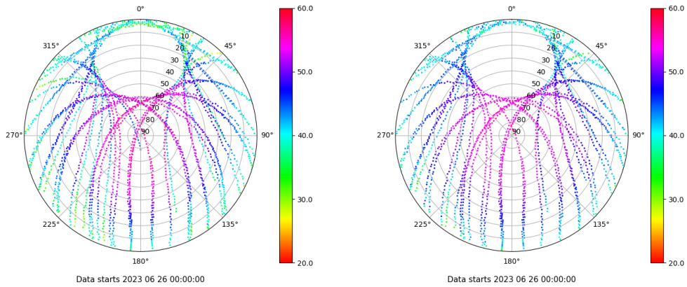
Skyplot for station XIXO. Signal to Noise S1C Data file XIXO00ESP_R_2023177.xtr Skyplot for station XIXO. Signal to Noise S2C Data file XIXO00ESP_R_2023177.xtr
