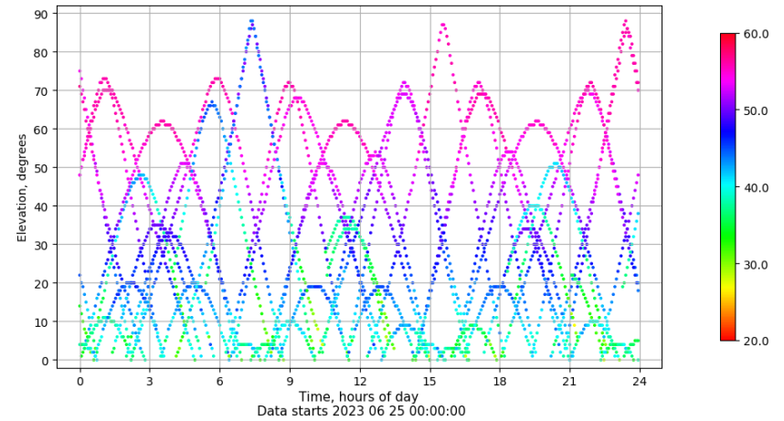
Time-elevation plot for station XIXO. Signal to Noise S1C Data file XIXO00ESP_R_2023176.xtr
