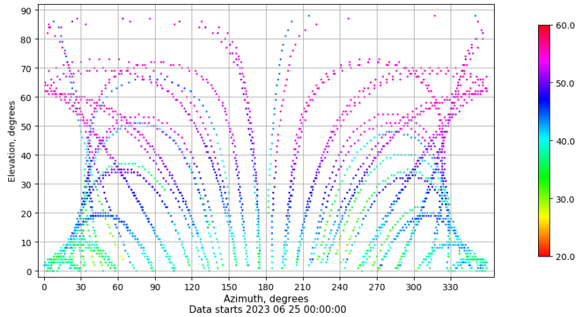
Azimuth-elevation plot for station XIXO. Signal to Noise S1C Data file XIXO00ESP_R_2023176.xtr
