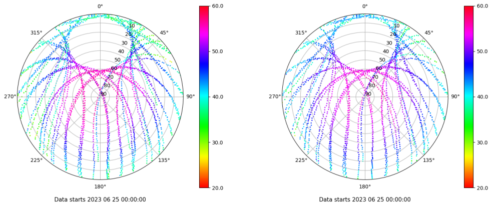
Skyplot for station XIXO. Signal to Noise S1C Data file XIXO00ESP_R_2023176.xtr Skyplot for station XIXO. Signal to Noise S2C Data file XIXO00ESP_R_2023176.xtr
