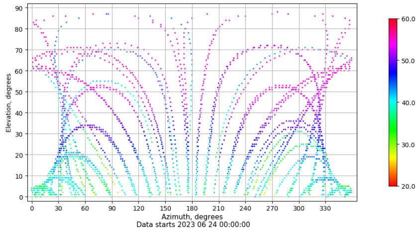
Azimuth-elevation plot for station XIXO. Signal to Noise S1C Data file XIXO00ESP_R_2023175.xtr
