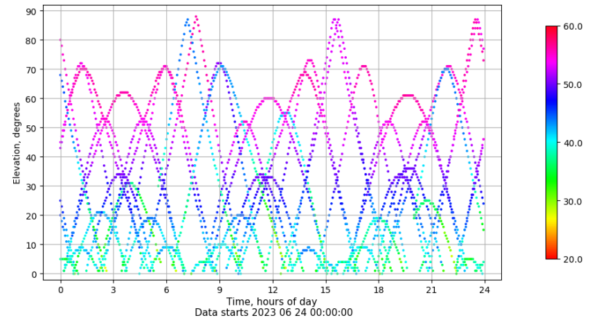
Time-elevation plot for station XIXO. Signal to Noise S1C Data file XIXO00ESP_R_2023175.xtr
