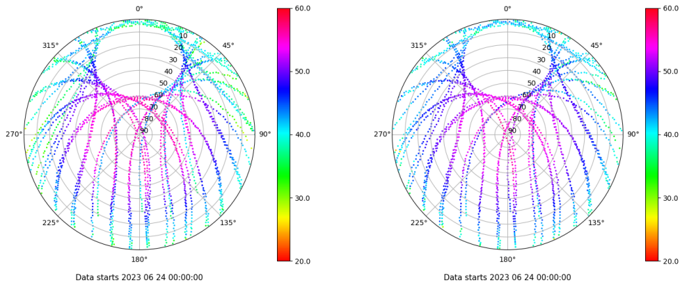
Skyplot for station XIXO. Signal to Noise S1C Data file XIXO00ESP_R_2023175.xtr Skyplot for station XIXO. Signal to Noise S2C Data file XIXO00ESP_R_2023175.xtr
