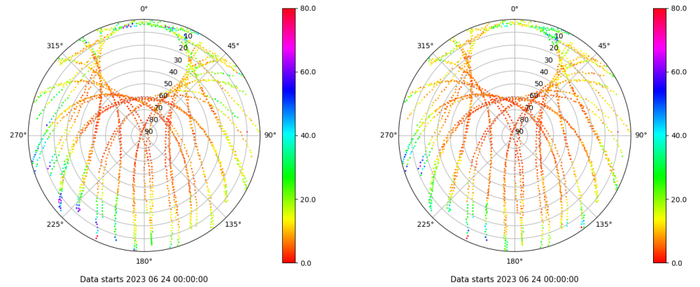
Skyplot for station XIXO. Parameter M1C Data file XIXO00ESP_R_2023175.xtr Skyplot for station XIXO. Parameter M2C Data file XIXO00ESP_R_2023175.xtr
