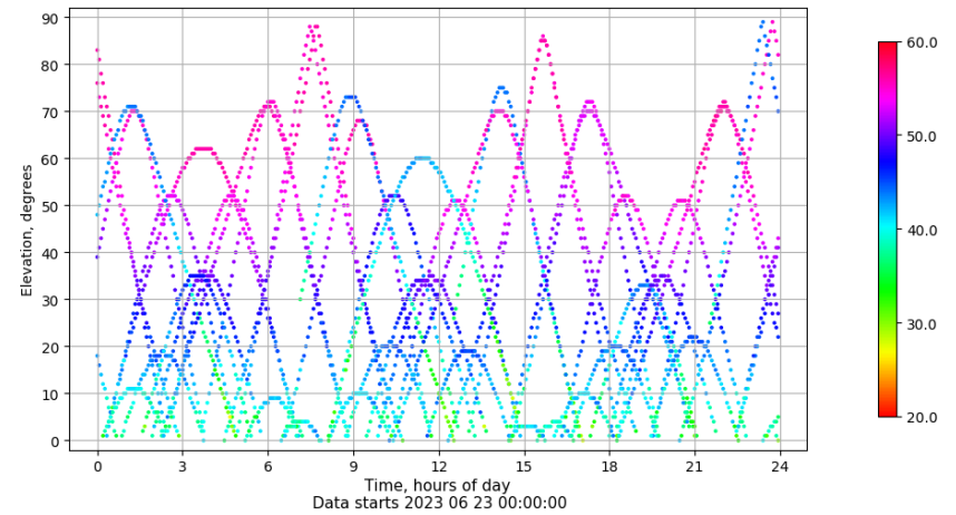
Time-elevation plot for station XIXO. Signal to Noise S1C Data file XIXO00ESP_R_2023174.xtr
