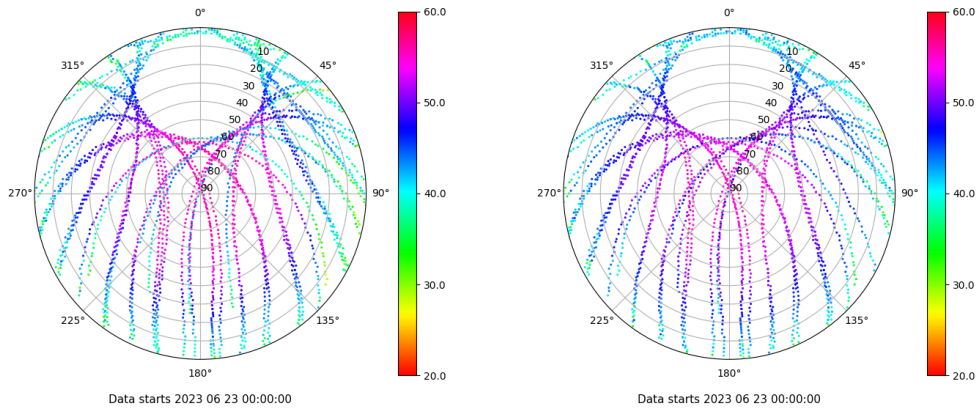
Skyplot for station XIXO. Signal to Noise S1C Data file XIXO00ESP_R_2023174.xtr Skyplot for station XIXO. Signal to Noise S2C Data file XIXO00ESP_R_2023174.xtr
