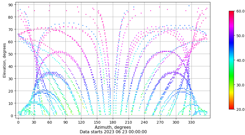
Azimuth-elevation plot for station XIXO. Signal to Noise S1C Data file XIXO00ESP_R_2023174.xtr
