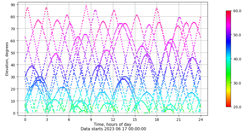
Time-elevation plot for station XIXO. Signal to Noise S1C Data file XIXO00ESP_R_2023168.xtr
