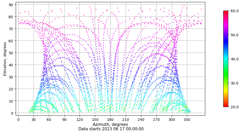
Azimuth-elevation plot for station XIXO. Signal to Noise S1C Data file XIXO00ESP_R_2023168.xtr
