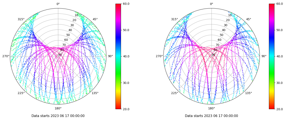
Skyplot for station XIXO. Signal to Noise S1C Data file XIXO00ESP_R_2023168.xtr Skyplot for station XIXO. Signal to Noise S2S Data file XIXO00ESP_R_2023168.xtr
