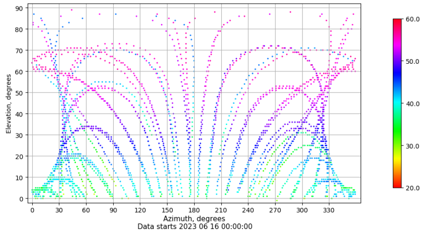
Azimuth-elevation plot for station XIXO. Signal to Noise S1C Data file XIXO00ESP_R_2023167.xtr
