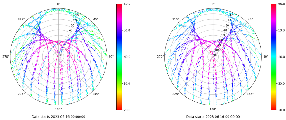
Skyplot for station XIXO. Signal to Noise S1C Data file XIXO00ESP_R_2023167.xtr Skyplot for station XIXO. Signal to Noise S2C Data file XIXO00ESP_R_2023167.xtr
