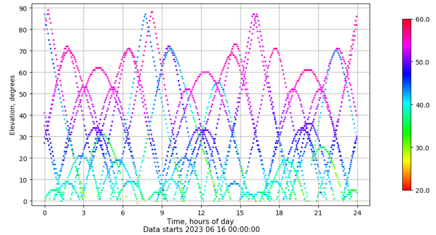
Time-elevation plot for station XIXO. Signal to Noise S1C Data file XIXO00ESP_R_2023167.xtr
