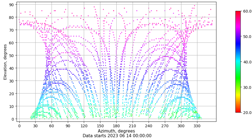
Azimuth-elevation plot for station XIXO. Signal to Noise S1C Data file XIXO00ESP_R_2023165.xtr
