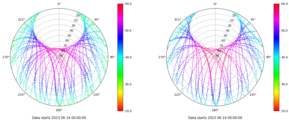
Skyplot for station XIXO. Signal to Noise S1C Data file XIXO00ESP_R_2023165.xtr Skyplot for station XIXO. Signal to Noise S2S Data file XIXO00ESP_R_2023165.xtr
