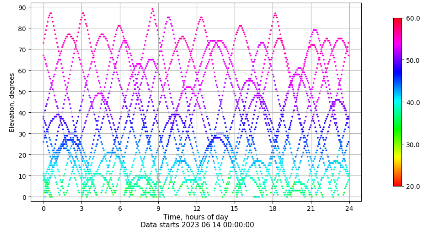
Time-elevation plot for station XIXO. Signal to Noise S1C Data file XIXO00ESP_R_2023165.xtr
