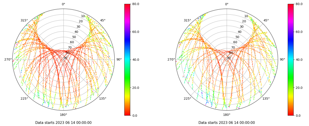
Skyplot for station XIXO. Parameter M1C Data file XIXO00ESP_R_2023165.xtr Skyplot for station XIXO. Parameter M2S Data file XIXO00ESP_R_2023165.xtr
