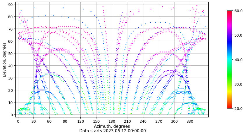
Azimuth-elevation plot for station XIXO. Signal to Noise S1C Data file XIXO00ESP_R_2023163.xtr
