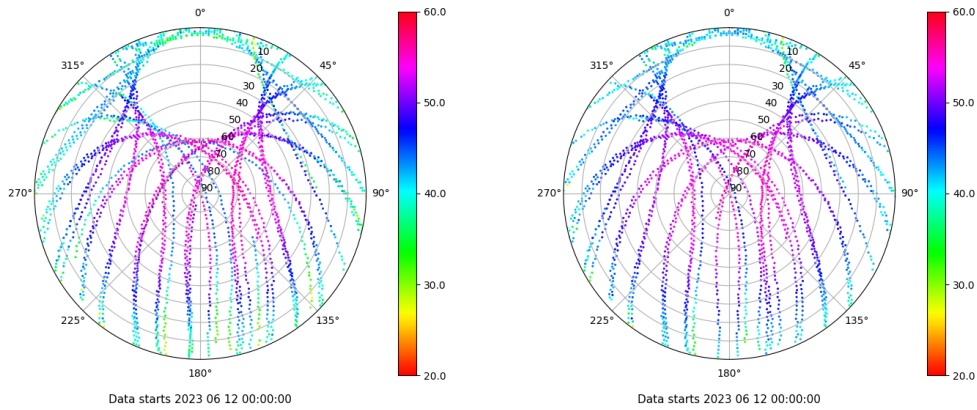
Skyplot for station XIXO. Signal to Noise S1C Data file XIXO00ESP_R_2023163.xtr Skyplot for station XIXO. Signal to Noise S2C Data file XIXO00ESP_R_2023163.xtr
