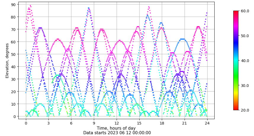
Time-elevation plot for station XIXO. Signal to Noise S1C Data file XIXO00ESP_R_2023163.xtr
