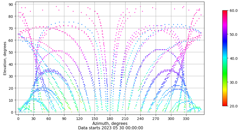
Azimuth-elevation plot for station XIXO. Signal to Noise S1C Data file XIXO00ESP_R_2023150.xtr
