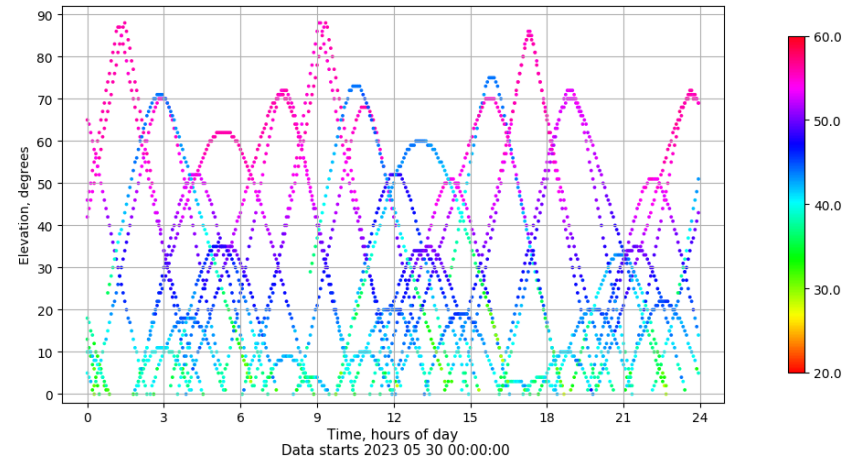
Time-elevation plot for station XIXO. Signal to Noise S1C Data file XIXO00ESP_R_2023150.xtr
