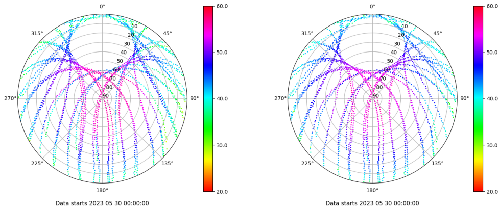
Skyplot for station XIXO. Signal to Noise S1C Data file XIXO00ESP_R_2023150.xtr Skyplot for station XIXO. Signal to Noise S2C Data file XIXO00ESP_R_2023150.xtr
