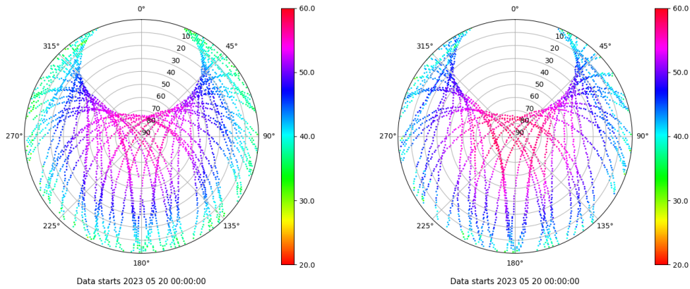
Skyplot for station XIXO. Signal to Noise S1C Data file XIXO00ESP_R_2023140.xtr Skyplot for station XIXO. Signal to Noise S2S Data file XIXO00ESP_R_2023140.xtr
