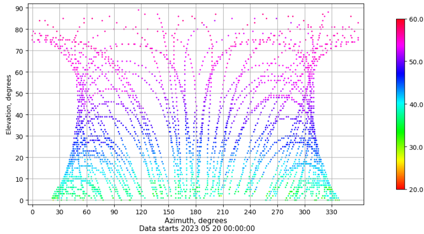
Azimuth-elevation plot for station XIXO. Signal to Noise S1C Data file XIXO00ESP_R_2023140.xtr
