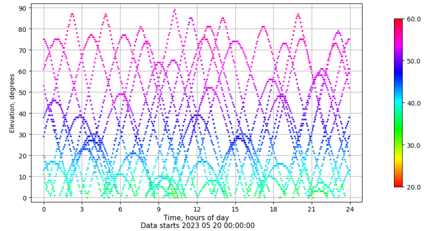
Time-elevation plot for station XIXO. Signal to Noise S1C Data file XIXO00ESP_R_2023140.xtr
