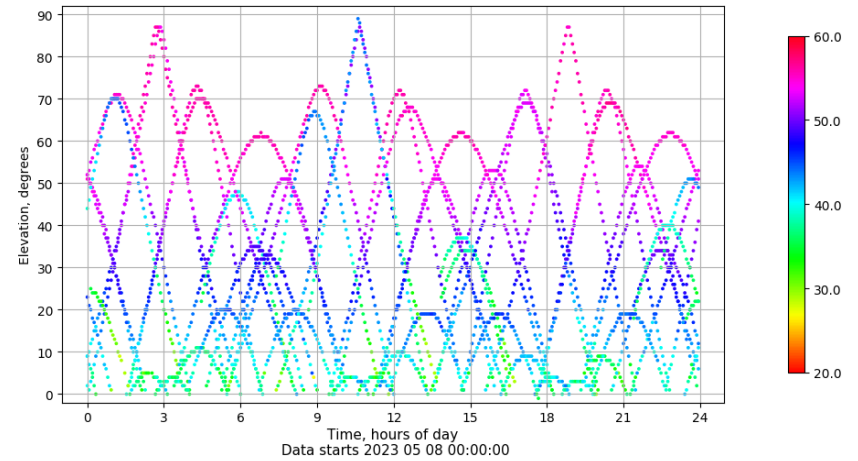
Time-elevation plot for station XIXO. Signal to Noise S1C Data file XIXO00ESP_R_2023128.xtr
