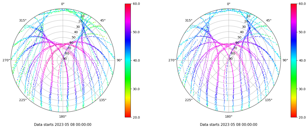
Skyplot for station XIXO. Signal to Noise S1C Data file XIXO00ESP_R_2023128.xtr Skyplot for station XIXO. Signal to Noise S2C Data file XIXO00ESP_R_2023128.xtr
