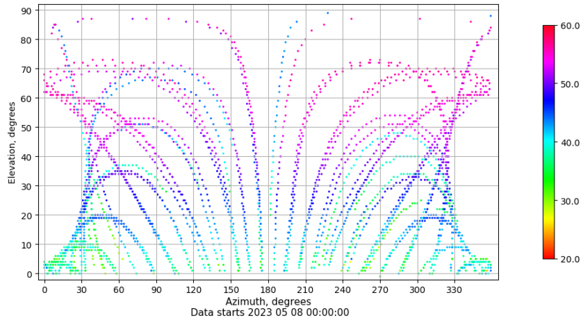
Azimuth-elevation plot for station XIXO. Signal to Noise S1C Data file XIXO00ESP_R_2023128.xtr
