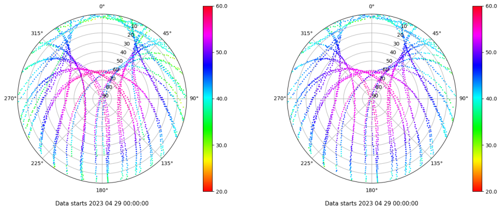
Skyplot for station XIXO. Signal to Noise S1C Data file XIXO00ESP_R_2023119.xtr Skyplot for station XIXO. Signal to Noise S2C Data file XIXO00ESP_R_2023119.xtr
