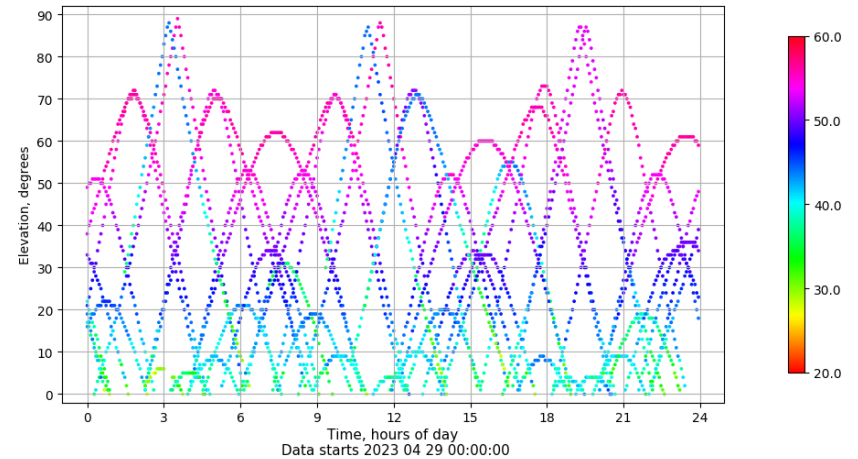
Time-elevation plot for station XIXO. Signal to Noise S1C Data file XIXO00ESP_R_2023119.xtr
