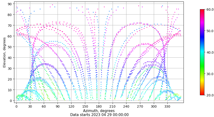
Azimuth-elevation plot for station XIXO. Signal to Noise S1C Data file XIXO00ESP_R_2023119.xtr
