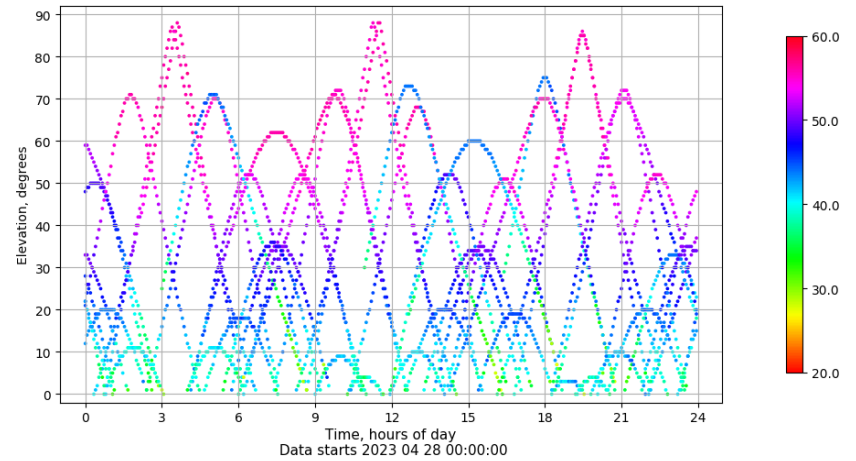
Time-elevation plot for station XIXO. Signal to Noise S1C Data file XIXO00ESP_R_2023118.xtr
