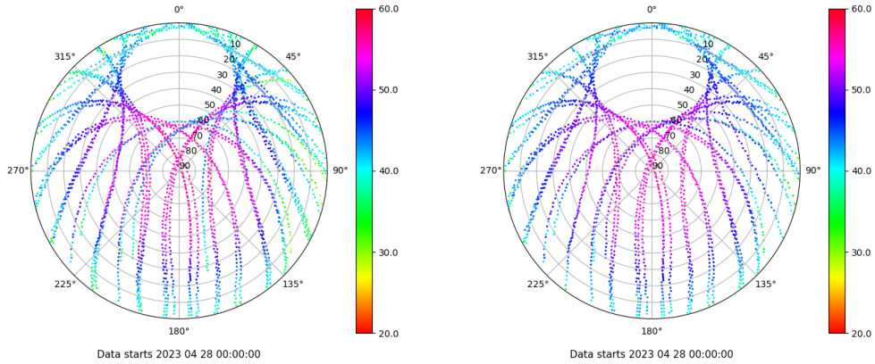
Skyplot for station XIXO. Signal to Noise S1C Data file XIXO00ESP_R_2023118.xtr Skyplot for station XIXO. Signal to Noise S2C Data file XIXO00ESP_R_2023118.xtr
