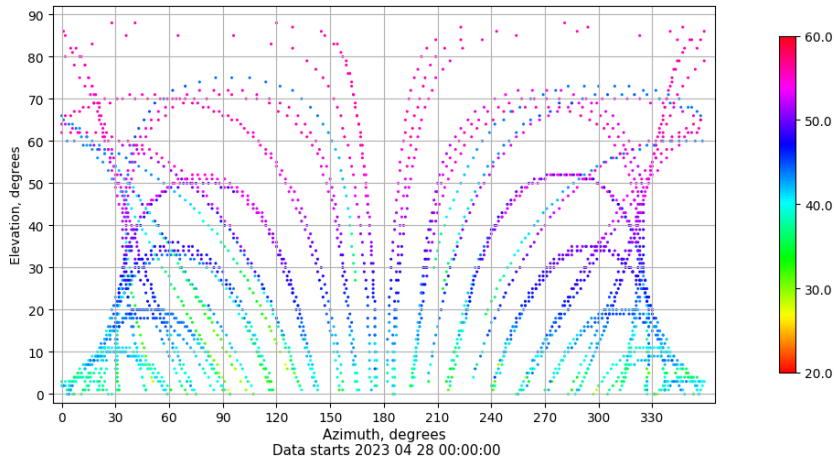
Azimuth-elevation plot for station XIXO. Signal to Noise S1C Data file XIXO00ESP_R_2023118.xtr
