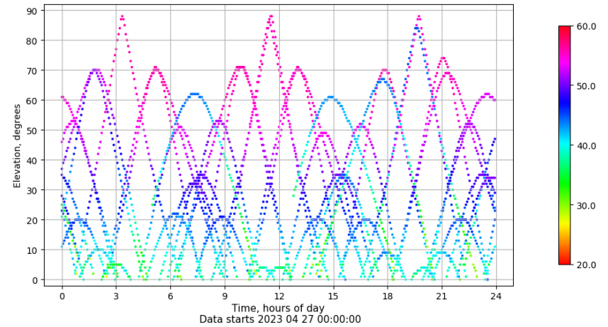
Time-elevation plot for station XIXO. Signal to Noise S1C Data file XIXO00ESP_R_2023117.xtr
