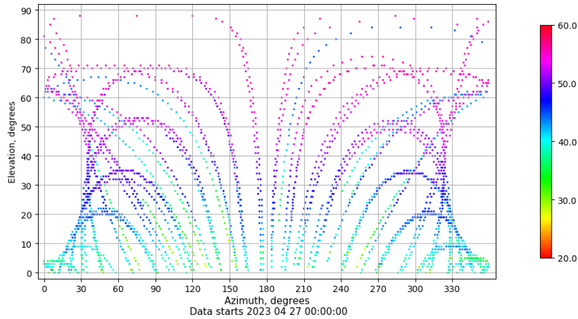
Azimuth-elevation plot for station XIXO. Signal to Noise S1C Data file XIXO00ESP_R_2023117.xtr
