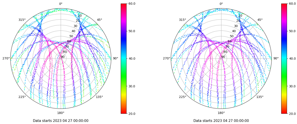
Skyplot for station XIXO. Signal to Noise S1C Data file XIXO00ESP_R_2023117.xtr Skyplot for station XIXO. Signal to Noise S2C Data file XIXO00ESP_R_2023117.xtr
