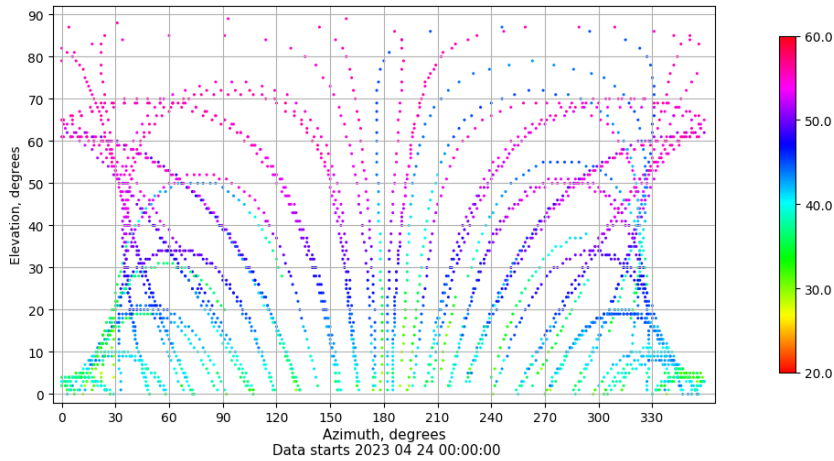
Azimuth-elevation plot for station XIXO. Signal to Noise S1C Data file XIXO00ESP_R_2023114.xtr
