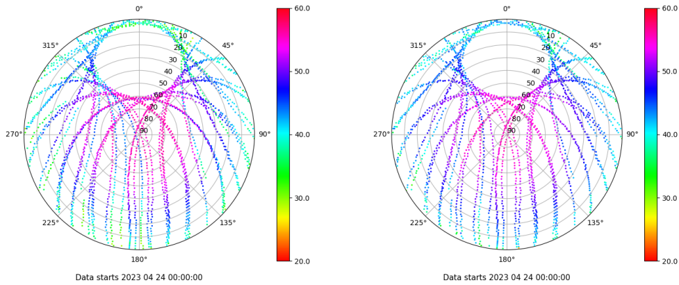
Skyplot for station XIXO. Signal to Noise S1C Data file XIXO00ESP_R_2023114.xtr Skyplot for station XIXO. Signal to Noise S2C Data file XIXO00ESP_R_2023114.xtr
