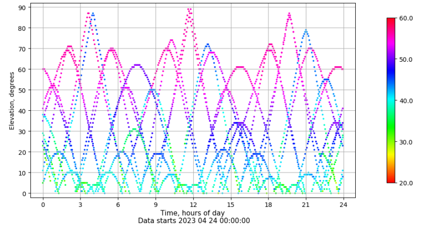
Time-elevation plot for station XIXO. Signal to Noise S1C Data file XIXO00ESP_R_2023114.xtr
