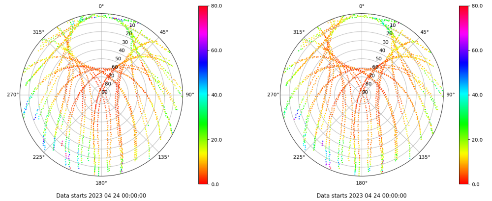
Skyplot for station XIXO. Parameter M1C Data file XIXO00ESP_R_2023114.xtr Skyplot for station XIXO. Parameter M2C Data file XIXO00ESP_R_2023114.xtr
