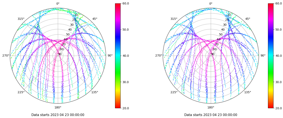
Skyplot for station XIXO. Signal to Noise S1C Data file XIXO00ESP_R_2023113.xtr Skyplot for station XIXO. Signal to Noise S2C Data file XIXO00ESP_R_2023113.xtr
