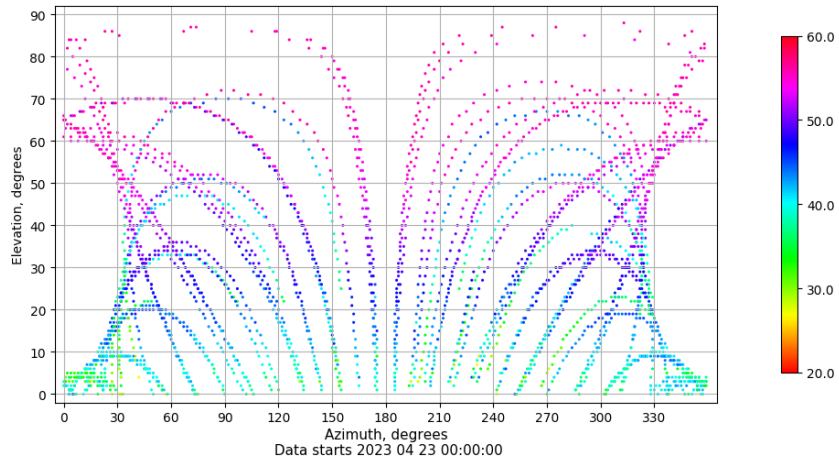
Azimuth-elevation plot for station XIXO. Signal to Noise S1C Data file XIXO00ESP_R_2023113.xtr
