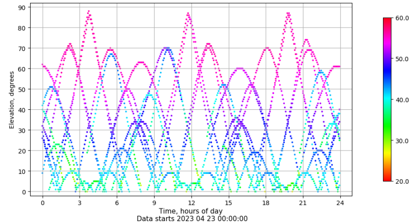
Time-elevation plot for station XIXO. Signal to Noise S1C Data file XIXO00ESP_R_2023113.xtr
