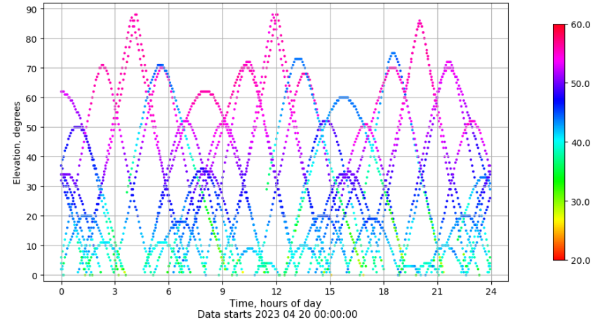
Time-elevation plot for station XIXO. Signal to Noise S1C Data file XIXO00ESP_R_2023110.xtr
