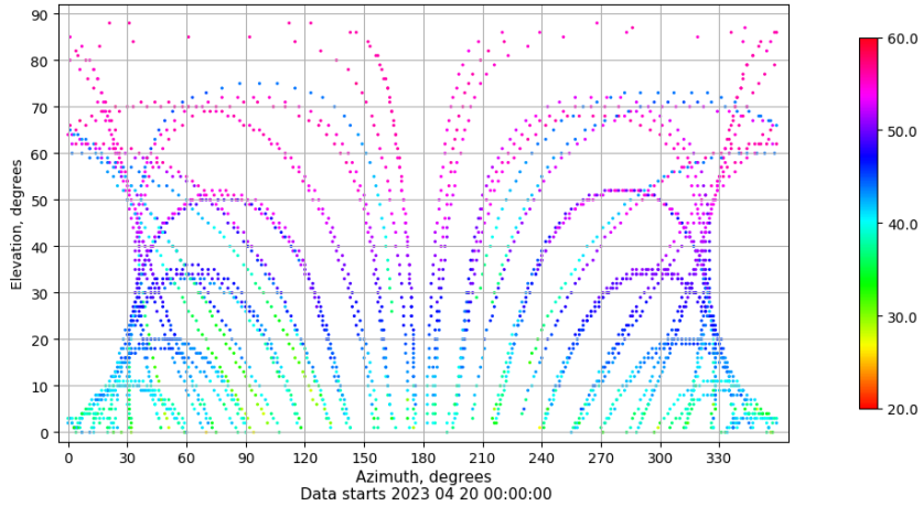
Azimuth-elevation plot for station XIXO. Signal to Noise S1C Data file XIXO00ESP_R_2023110.xtr
