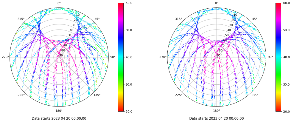
Skyplot for station XIXO. Signal to Noise S1C Data file XIXO00ESP_R_2023110.xtr Skyplot for station XIXO. Signal to Noise S2C Data file XIXO00ESP_R_2023110.xtr
