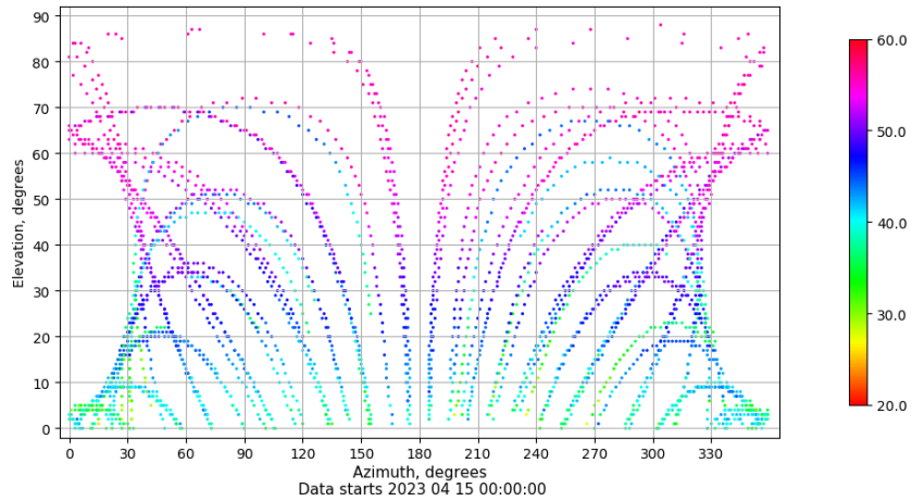
Azimuth-elevation plot for station XIXO. Signal to Noise S1C Data file XIXO00ESP_R_2023105.xtr
