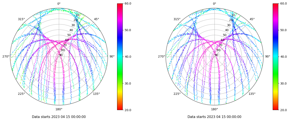
Skyplot for station XIXO. Signal to Noise S1C Data file XIXO00ESP_R_2023105.xtr Skyplot for station XIXO. Signal to Noise S2C Data file XIXO00ESP_R_2023105.xtr
