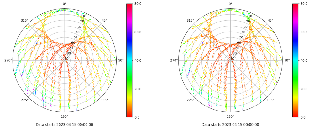
Skyplot for station XIXO. Parameter M1C Data file XIXO00ESP_R_2023105.xtr Skyplot for station XIXO. Parameter M2C Data file XIXO00ESP_R_2023105.xtr
