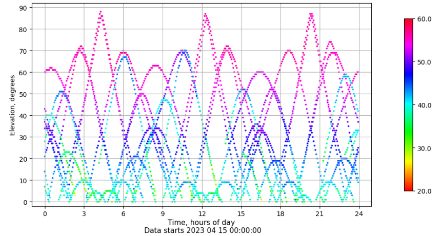
Time-elevation plot for station XIXO. Signal to Noise S1C Data file XIXO00ESP_R_2023105.xtr
