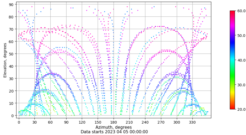
Azimuth-elevation plot for station XIXO. Signal to Noise S1C Data file XIXO00ESP_R_2023095.xtr
