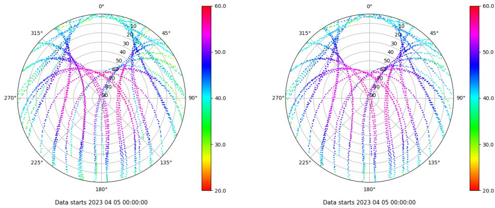
Skyplot for station XIXO. Signal to Noise S1C Data file XIXO00ESP_R_2023095.xtr Skyplot for station XIXO. Signal to Noise S2C Data file XIXO00ESP_R_2023095.xtr
