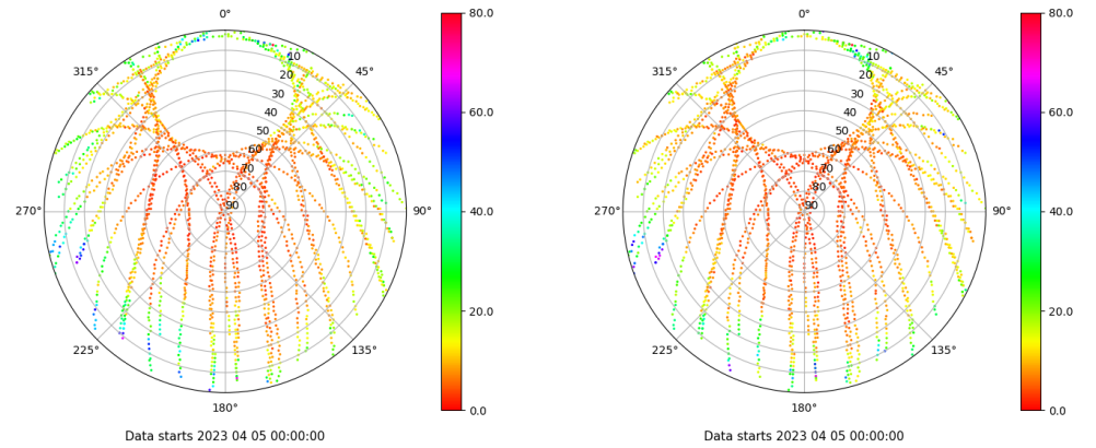
Skyplot for station XIXO. Parameter M1C Data file XIXO00ESP_R_2023095.xtr Skyplot for station XIXO. Parameter M2C Data file XIXO00ESP_R_2023095.xtr
