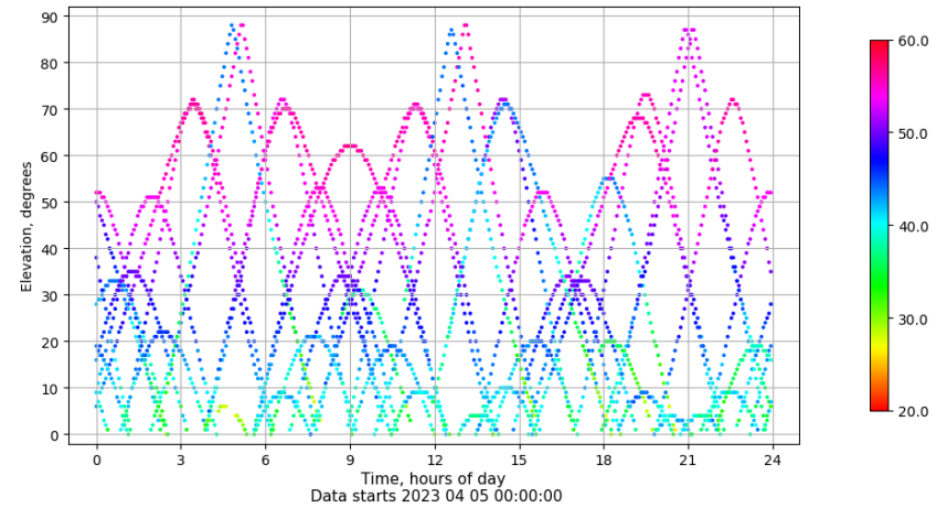
Time-elevation plot for station XIXO. Signal to Noise S1C Data file XIXO00ESP_R_2023095.xtr
