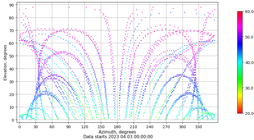
Azimuth-elevation plot for station XIXO. Signal to Noise S1C Data file XIXO00ESP_R_2023093.xtr
