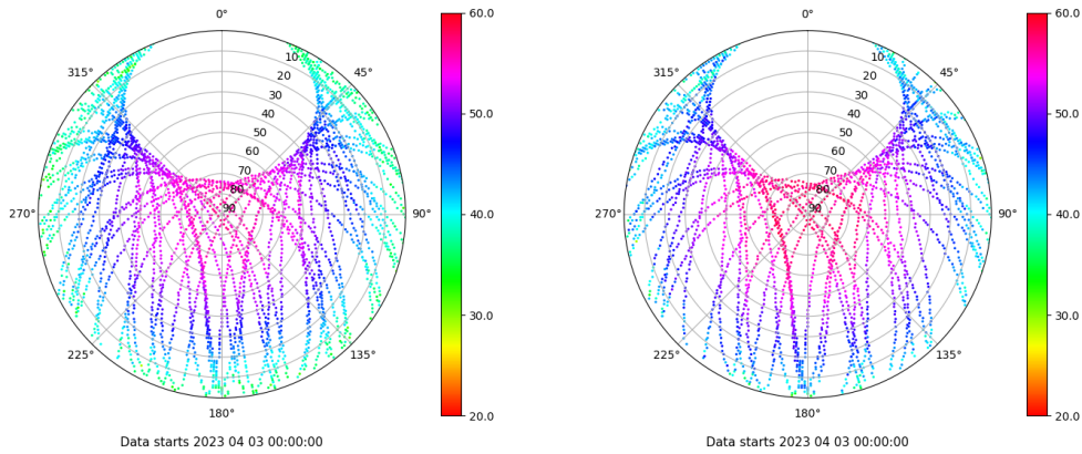
Skyplot for station XIXO. Signal to Noise S1C Data file XIXO00ESP_R_2023093.xtr Skyplot for station XIXO. Signal to Noise S2S Data file XIXO00ESP_R_2023093.xtr
