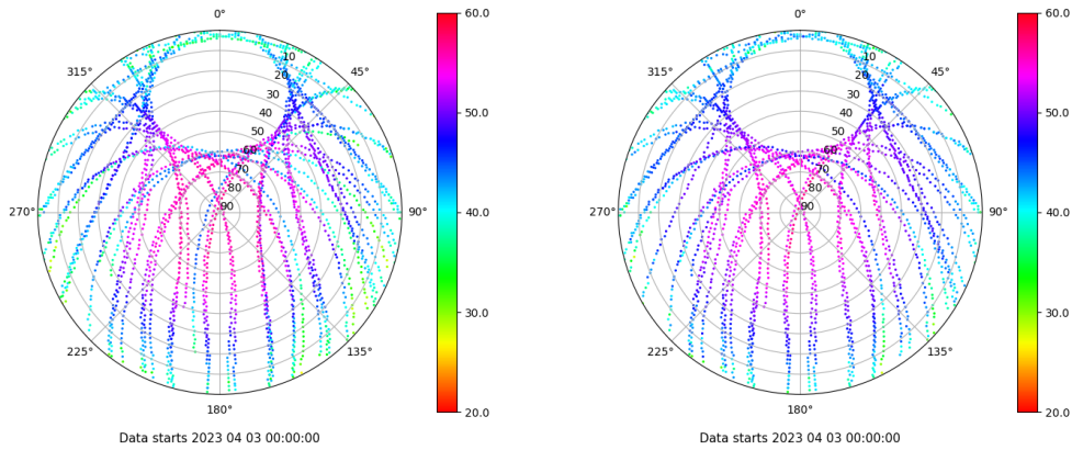
Skyplot for station XIXO. Signal to Noise S1C Data file XIXO00ESP_R_2023093.xtr Skyplot for station XIXO. Signal to Noise S2C Data file XIXO00ESP_R_2023093.xtr
