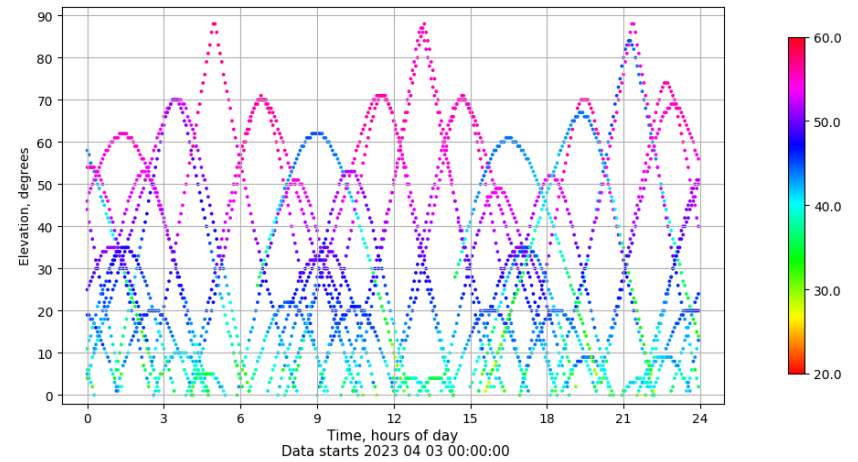
Time-elevation plot for station XIXO. Signal to Noise S1C Data file XIXO00ESP_R_2023093.xtr
