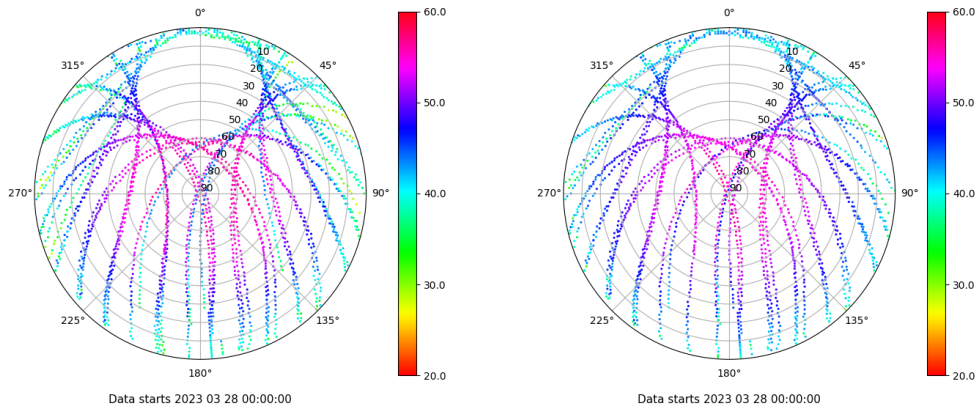
Skyplot for station XIXO. Signal to Noise S1C Data file XIXO00ESP_R_2023087.xtr Skyplot for station XIXO. Signal to Noise S2C Data file XIXO00ESP_R_2023087.xtr
