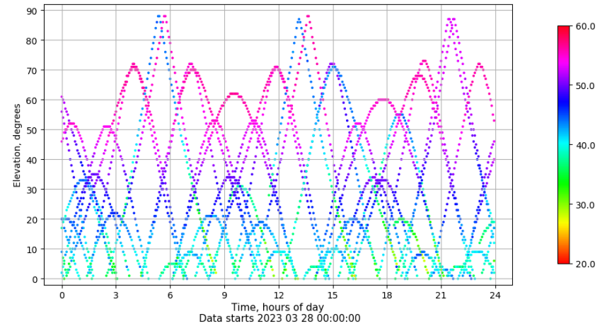
Time-elevation plot for station XIXO. Signal to Noise S1C Data file XIXO00ESP_R_2023087.xtr
