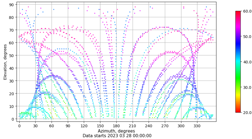
Azimuth-elevation plot for station XIXO. Signal to Noise S1C Data file XIXO00ESP_R_2023087.xtr
