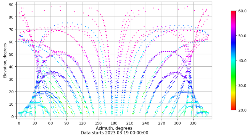
Azimuth-elevation plot for station XIXO. Signal to Noise S1C Data file XIXO00ESP_R_2023078.xtr
