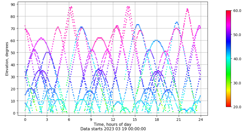
Time-elevation plot for station XIXO. Signal to Noise S1C Data file XIXO00ESP_R_2023078.xtr
