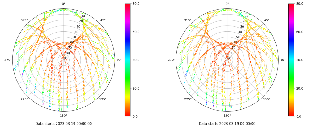
Skyplot for station XIXO. Parameter M1C Data file XIXO00ESP_R_2023078.xtr Skyplot for station XIXO. Parameter M2C Data file XIXO00ESP_R_2023078.xtr
