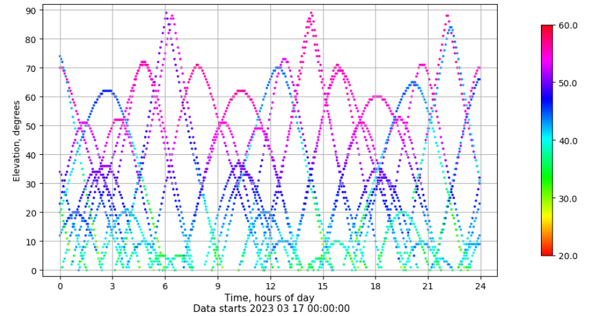
Time-elevation plot for station XIXO. Signal to Noise S1C Data file XIXO00ESP_R_2023076.xtr
