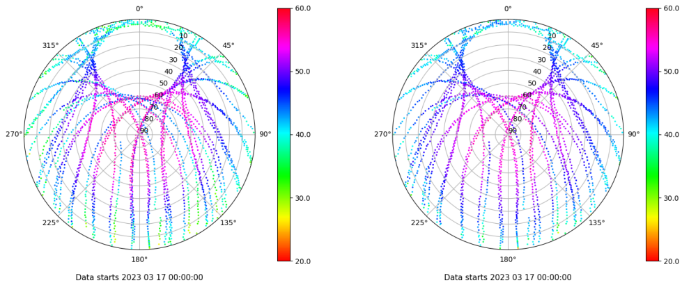
Skyplot for station XIXO. Signal to Noise S1C Data file XIXO00ESP_R_2023076.xtr Skyplot for station XIXO. Signal to Noise S2C Data file XIXO00ESP_R_2023076.xtr
