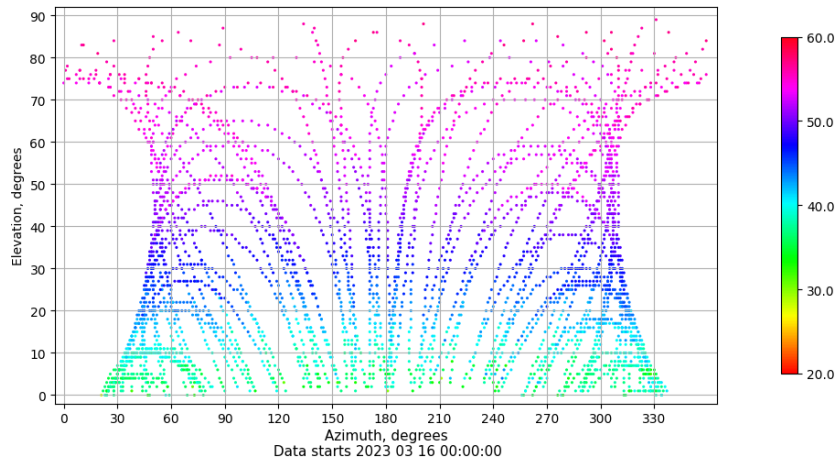
Azimuth-elevation plot for station XIXO. Signal to Noise S1C Data file XIXO00ESP_R_2023075.xtr
