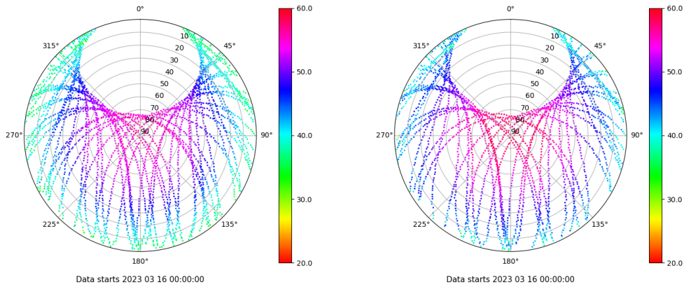
Skyplot for station XIXO. Signal to Noise S1C Data file XIXO00ESP_R_2023075.xtr Skyplot for station XIXO. Signal to Noise S2S Data file XIXO00ESP_R_2023075.xtr
