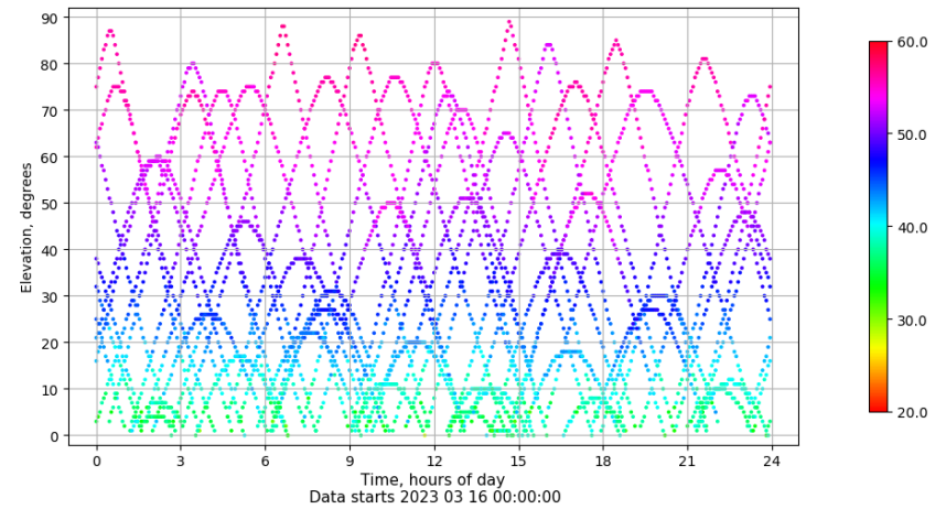
Time-elevation plot for station XIXO. Signal to Noise S1C Data file XIXO00ESP_R_2023075.xtr
