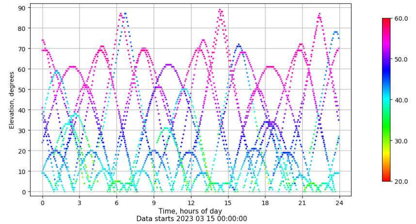
Time-elevation plot for station XIXO. Signal to Noise S1C Data file XIXO00ESP_R_2023074.xtr
