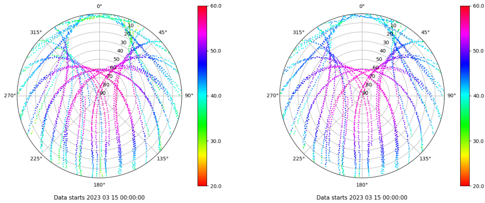
Skyplot for station XIXO. Signal to Noise S1C Data file XIXO00ESP_R_2023074.xtr Skyplot for station XIXO. Signal to Noise S2C Data file XIXO00ESP_R_2023074.xtr
