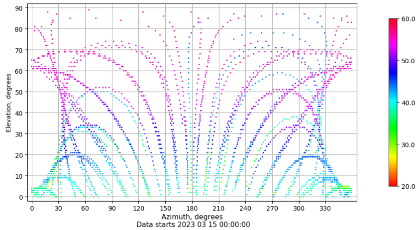
Azimuth-elevation plot for station XIXO. Signal to Noise S1C Data file XIXO00ESP_R_2023074.xtr
