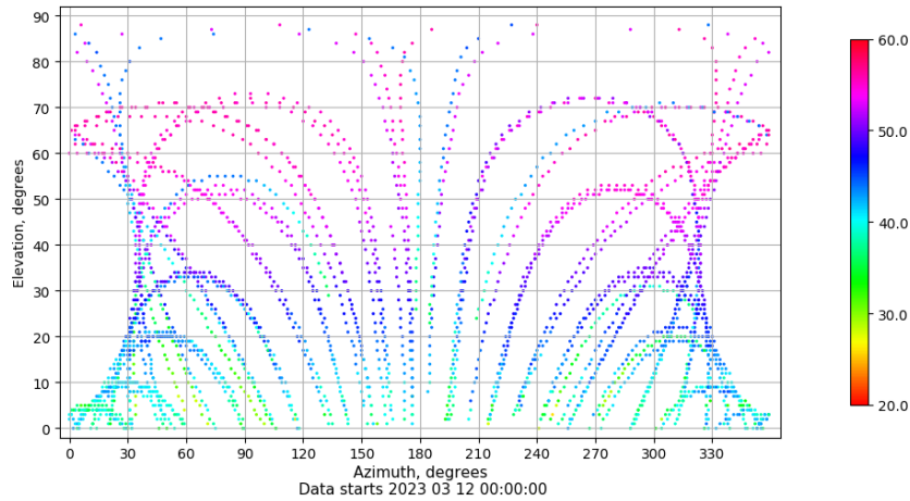
Azimuth-elevation plot for station XIXO. Signal to Noise S1C Data file XIXO00ESP_R_2023071.xtr
