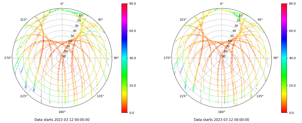
Skyplot for station XIXO. Parameter M1C Data file XIXO00ESP_R_2023071.xtr Skyplot for station XIXO. Parameter M2C Data file XIXO00ESP_R_2023071.xtr
