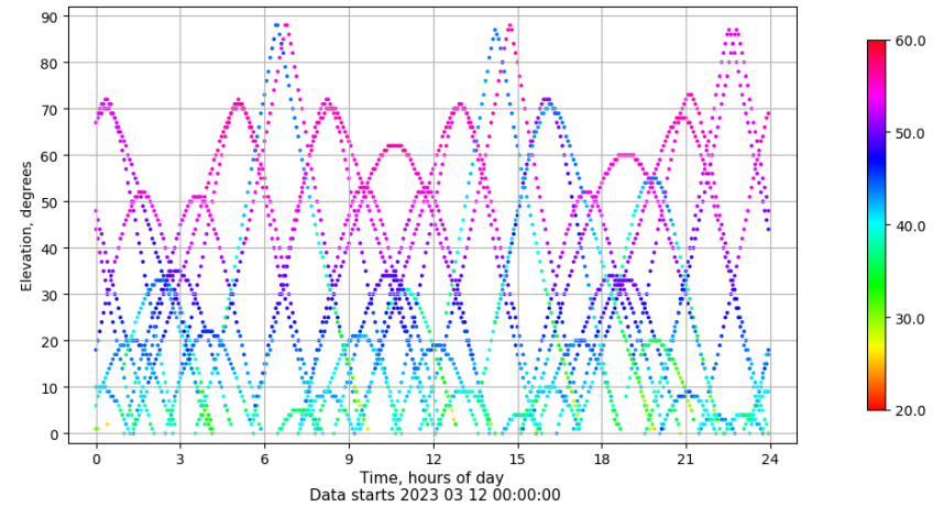
Time-elevation plot for station XIXO. Signal to Noise S1C Data file XIXO00ESP_R_2023071.xtr
