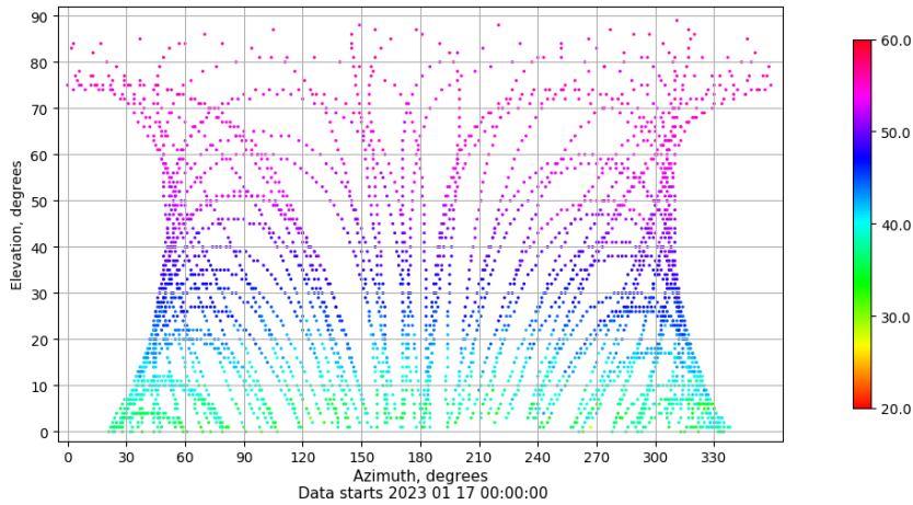
Azimuth-elevation plot for station XIXO. Signal to Noise S1C Data file XIXO00ESP_R_2023017.xtr
