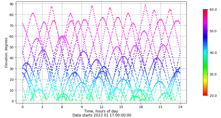
Time-elevation plot for station XIXO. Signal to Noise S1C Data file XIXO00ESP_R_2023017.xtr
