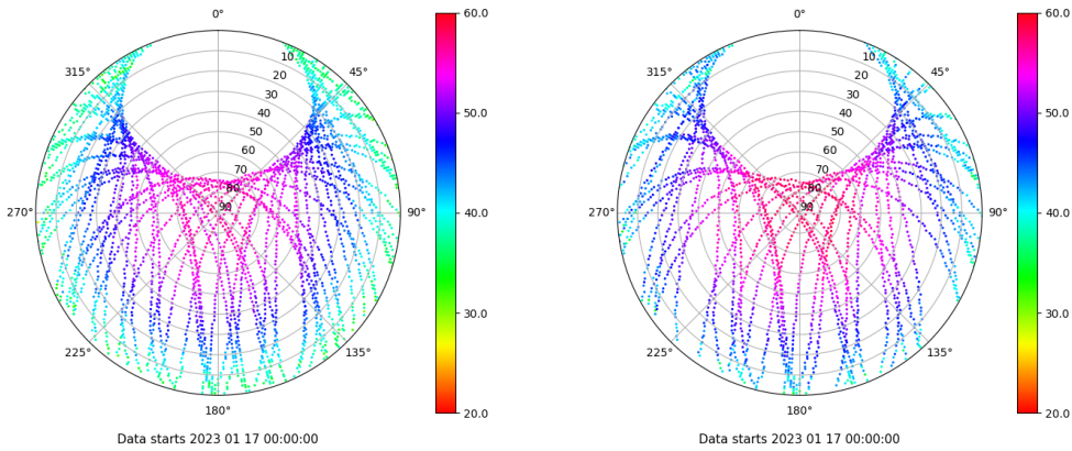
Skyplot for station XIXO. Signal to Noise S1C Data file XIXO00ESP_R_2023017.xtr Skyplot for station XIXO. Signal to Noise S2S Data file XIXO00ESP_R_2023017.xtr
