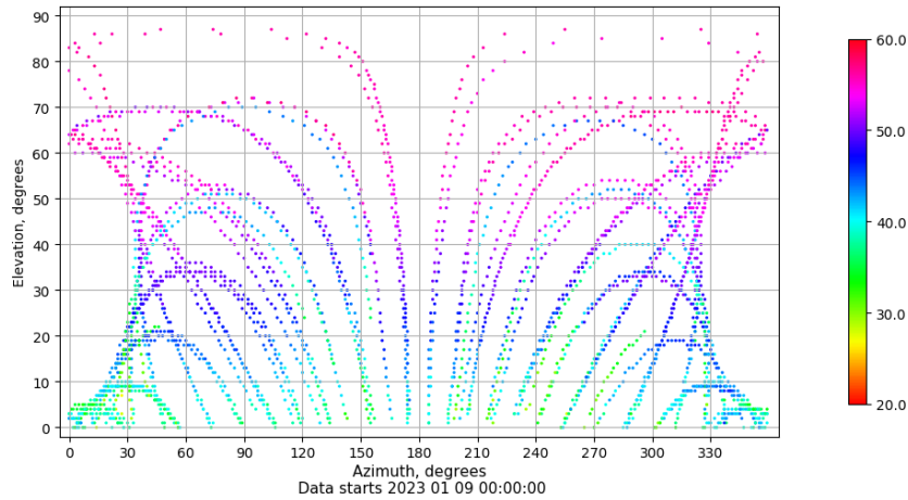
Azimuth-elevation plot for station XIXO. Signal to Noise S1C Data file XIXO00ESP_R_2023009.xtr
