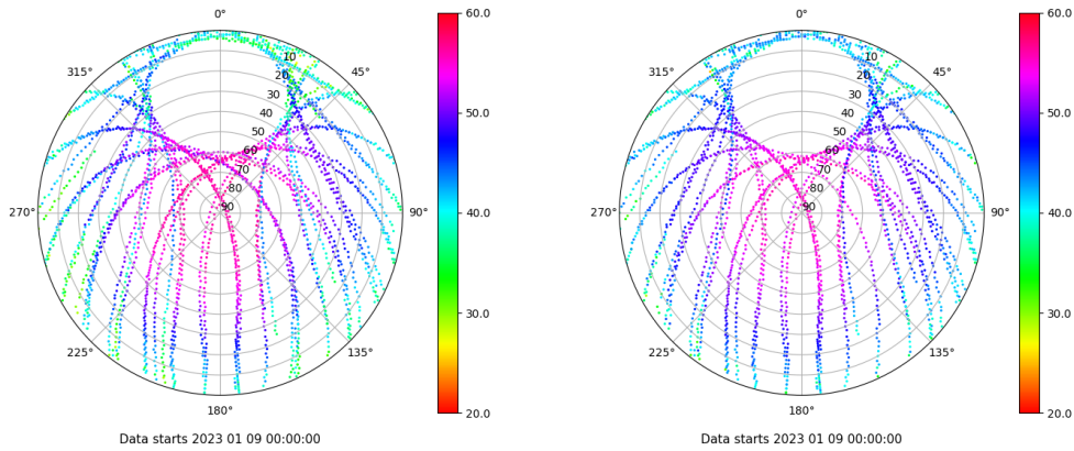
Skyplot for station XIXO. Signal to Noise S1C Data file XIXO00ESP_R_2023009.xtr Skyplot for station XIXO. Signal to Noise S2C Data file XIXO00ESP_R_2023009.xtr
