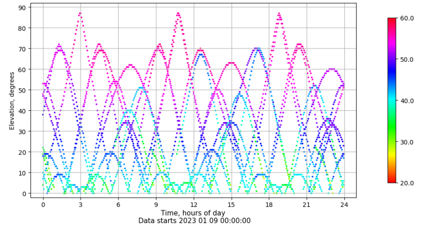
Time-elevation plot for station XIXO. Signal to Noise S1C Data file XIXO00ESP_R_2023009.xtr
